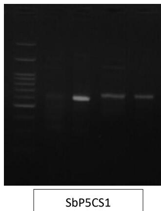
Figure 2. DNA polymorphism of the four citrus genotypes leaves amplified with primer proline.
