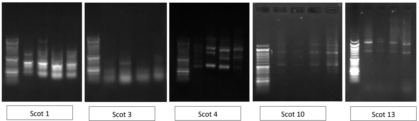
Figure 1. DNA polymorphism analysis of four citrus genotypes using five SCOT primers.
