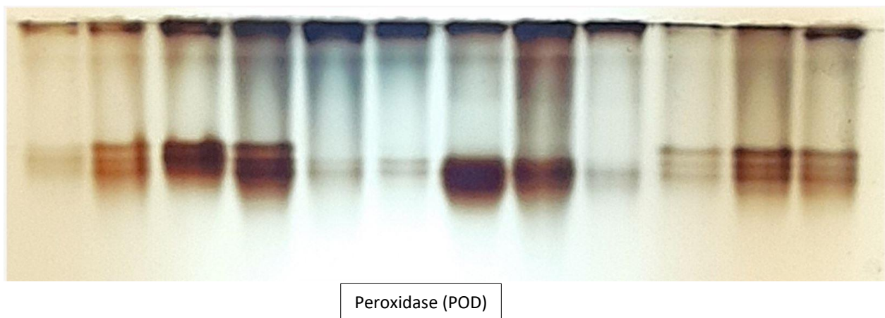
Figure 3. Electrophoresis of peroxidase of the four citrus genotypes leaves. Antioxidant enzyme activities (Peroxidase POD)
