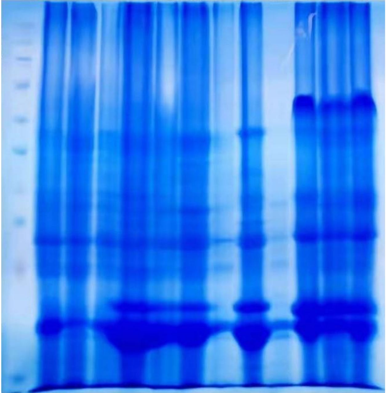
Figure 5. Protein electrophoresis of the four citrus genotype leaves. SDS-PAGE protein banding patterns of citrus leaves.
