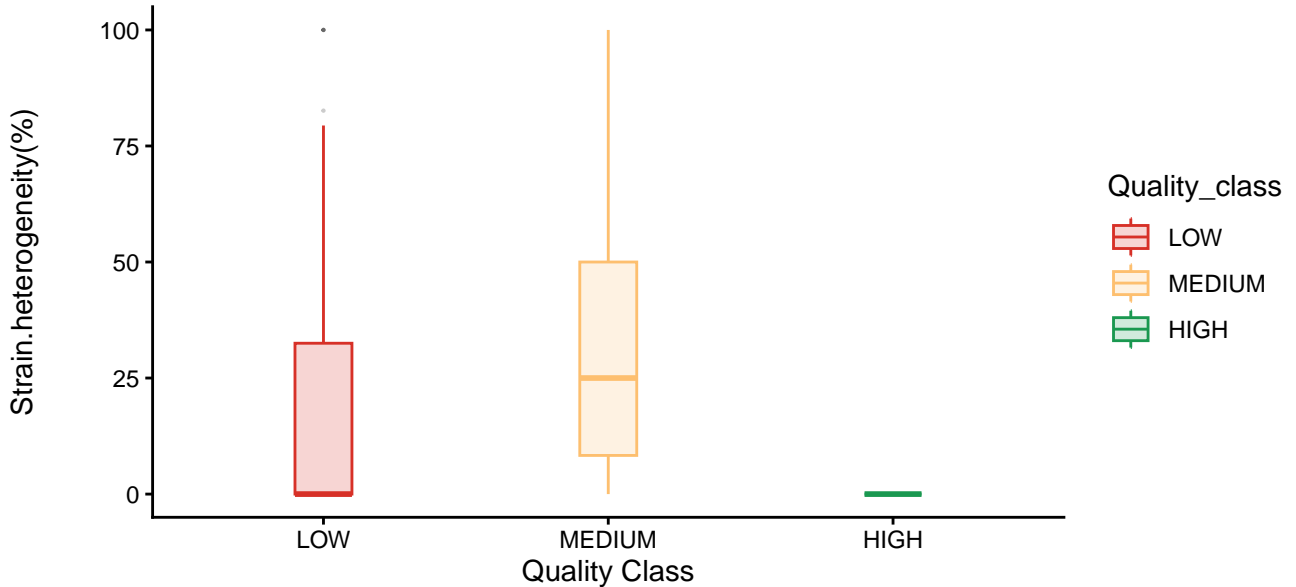
Strain heterogeneity by Quality Class
