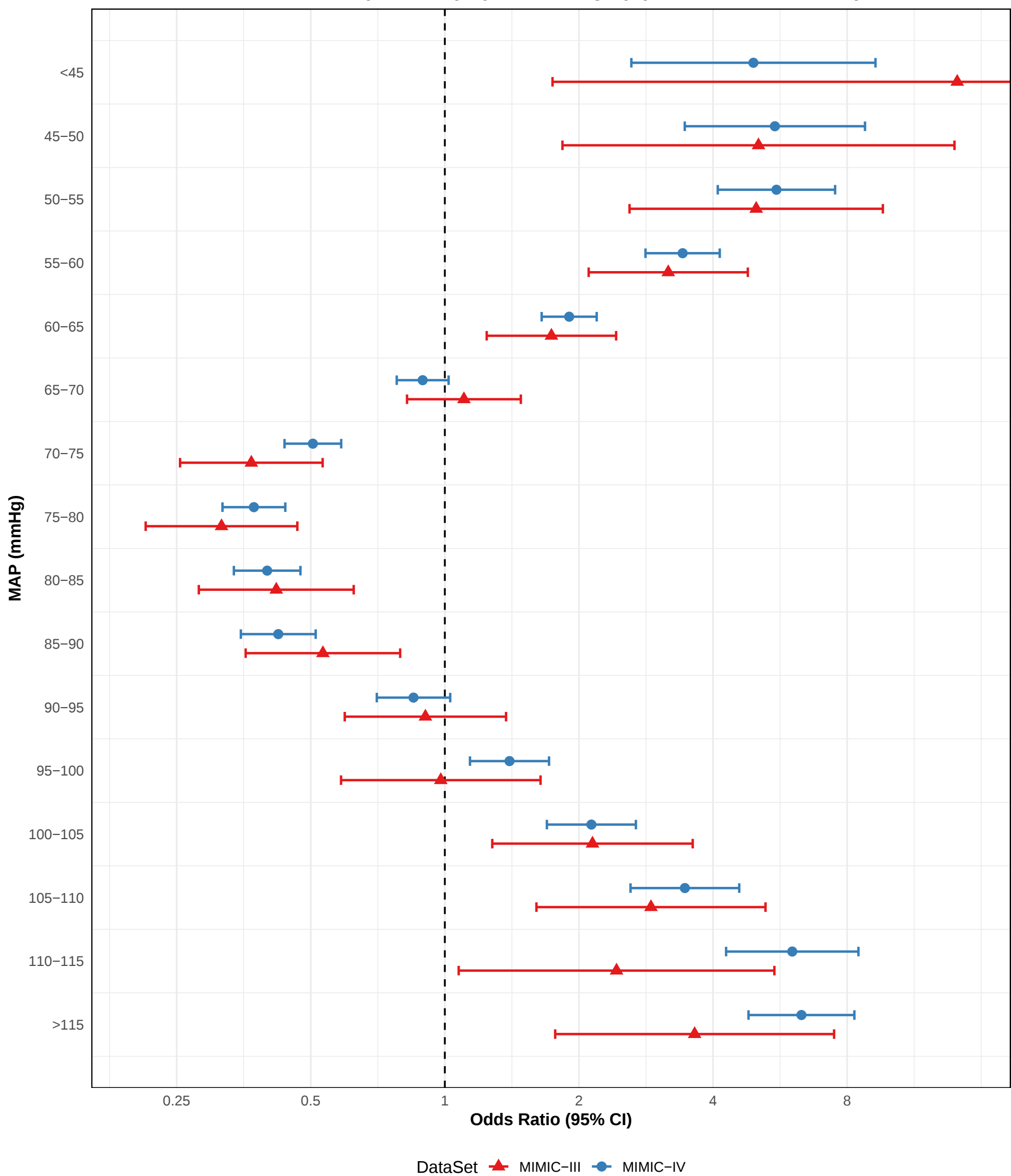
OR for 28-Day Mortality by MAP Category (MIMIC-III vs MIMIC-IV)
