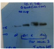
GDNF
