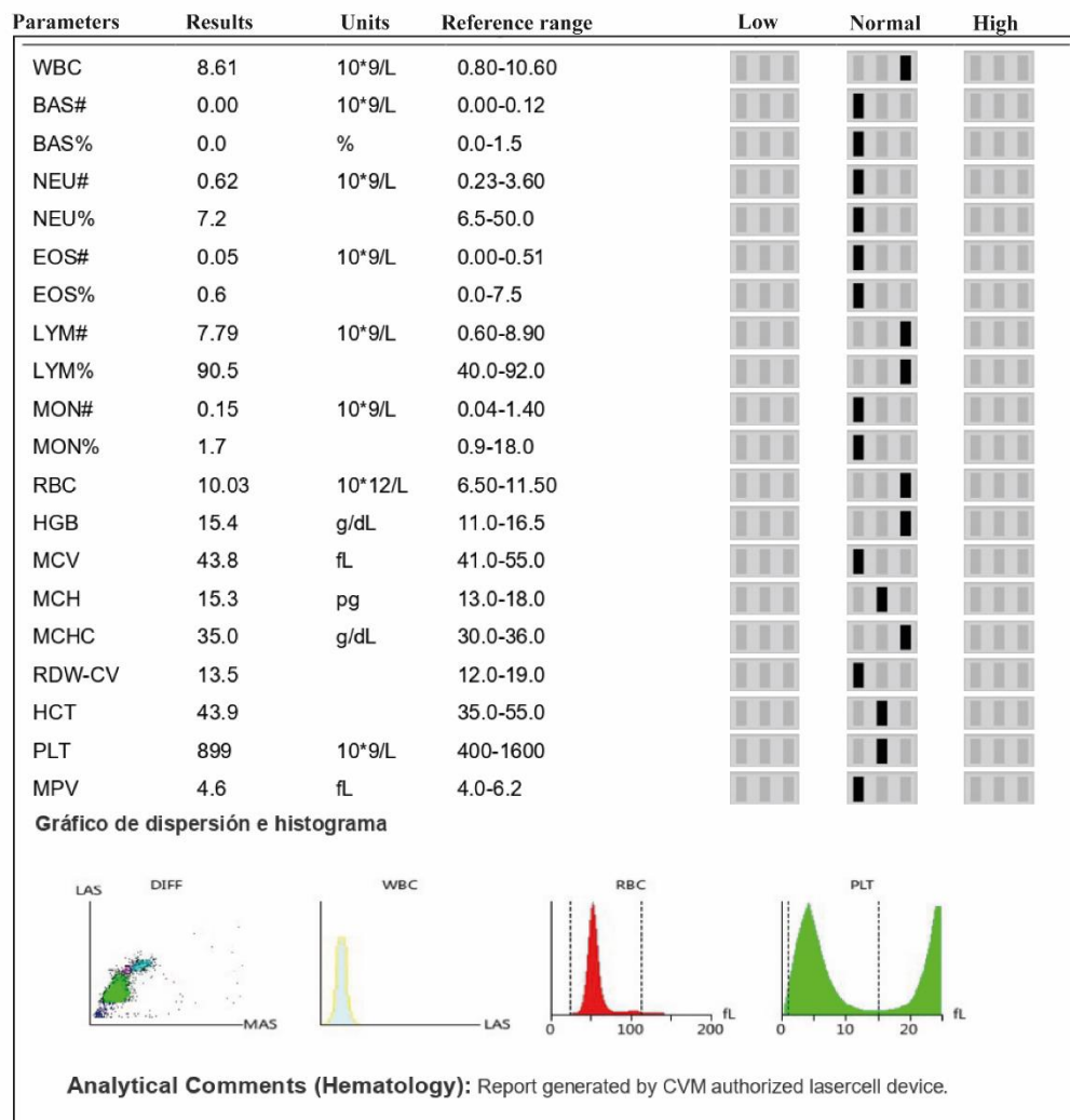
Figure S1. Blood analysis of previously MEMP treated and remitted tumor mouse 1-0. Mouse 1-0 was subjected to blood analysis after tumor remission following MEMP treatment and before to reinoculated it with the same cancer cell line MC-38-Luc. Samples were analyzed by Element HT5 hematology system (Scilvet Company).
