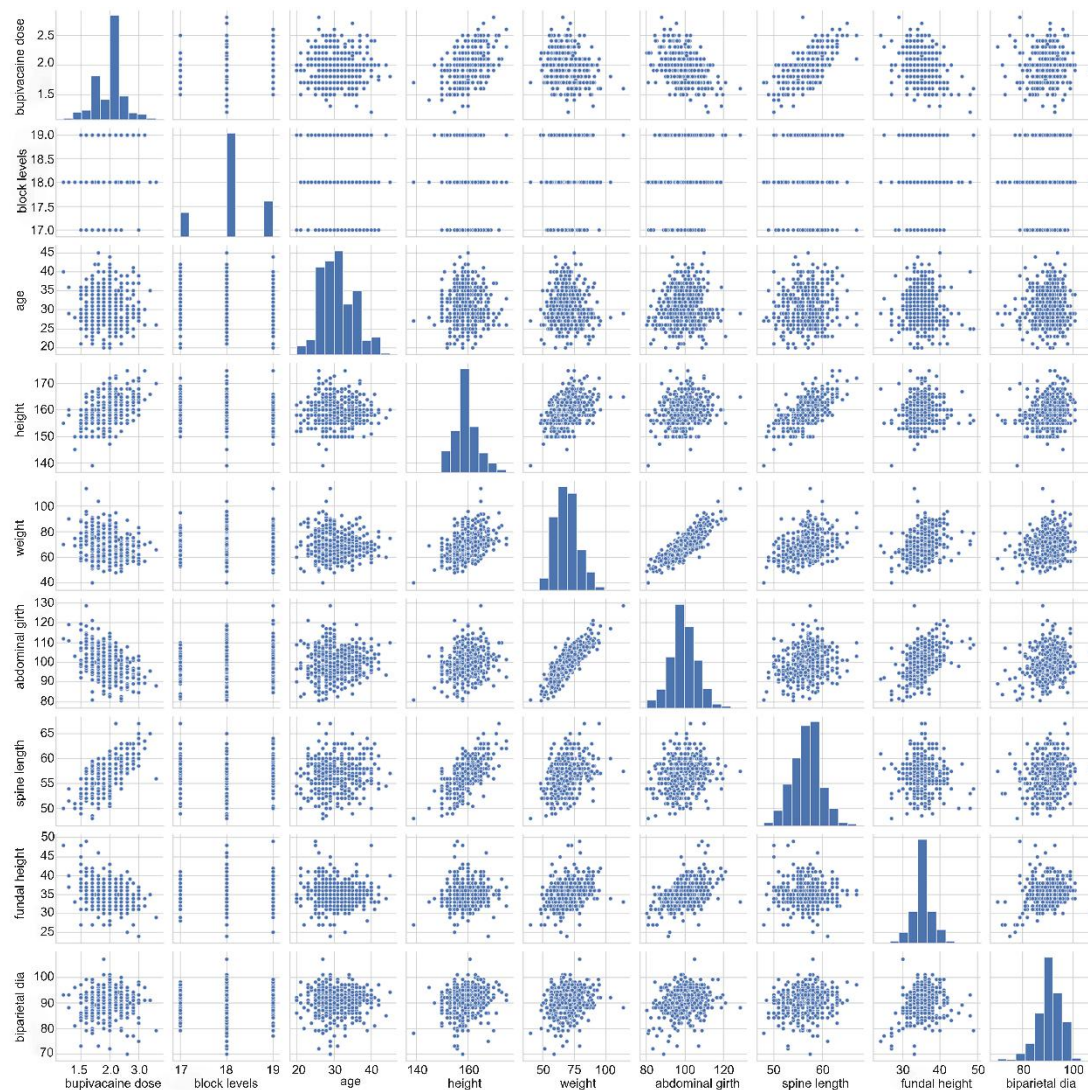
Fig 1. Visual analysis diagram of correlation between physical variables and intrathecal bupivacaine dose for the parturients with block levels between T4 and T6.
