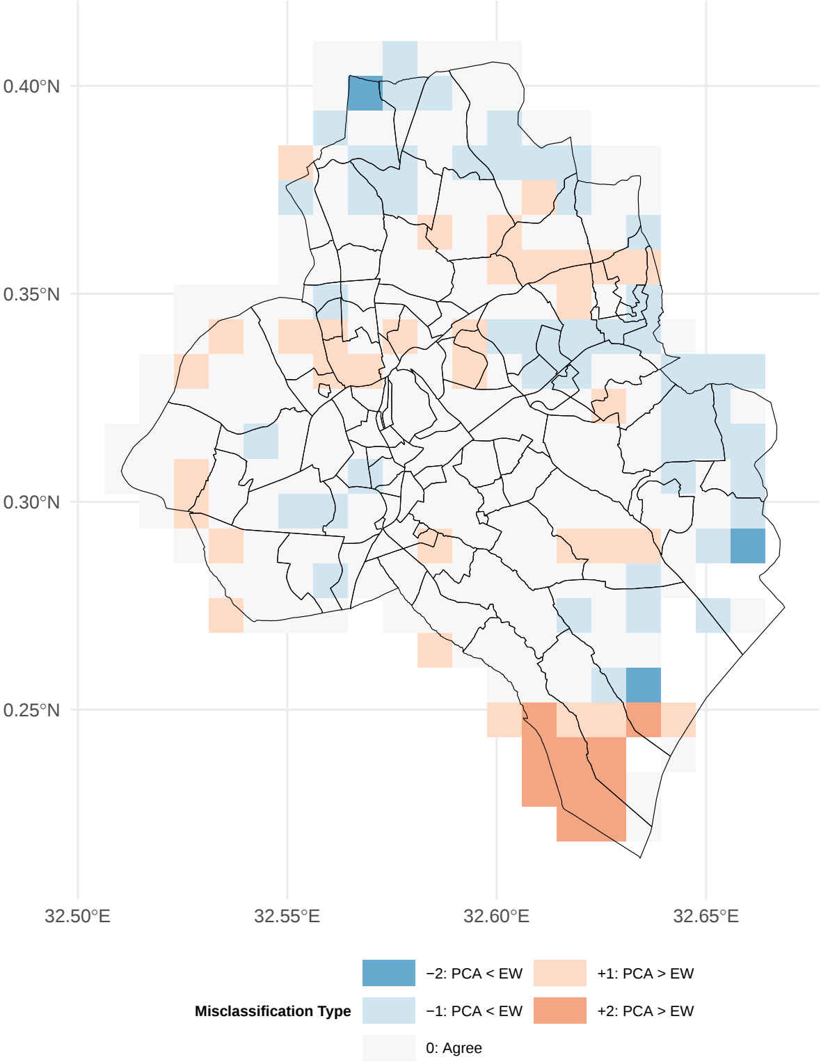
Directional Misclassification Map (Quartile-Based) Signed Difference in Vulnerability Classification (PCA – Equal-Weight)
