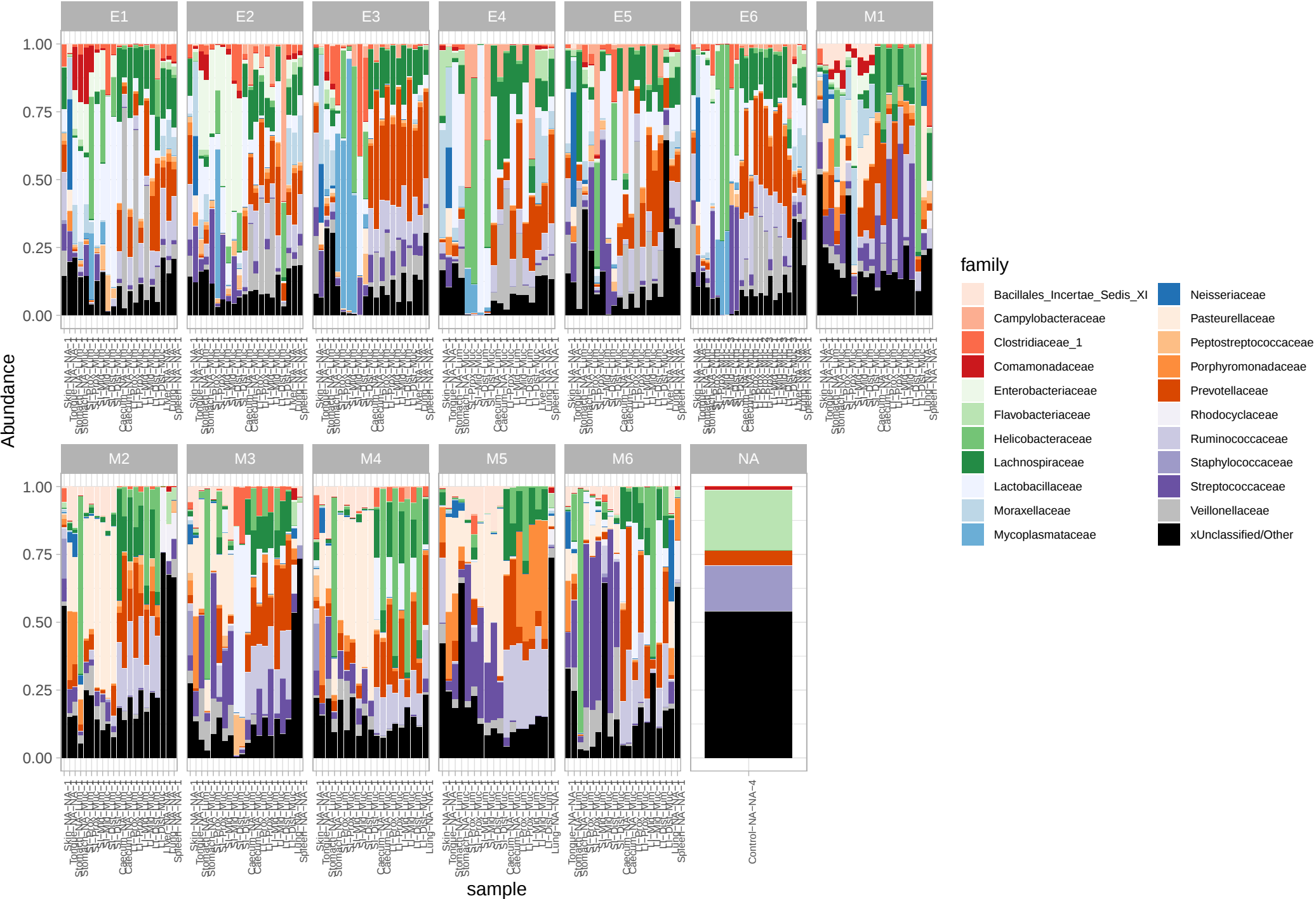
Bacterial families with relative abundance of >20% in any of the samples
