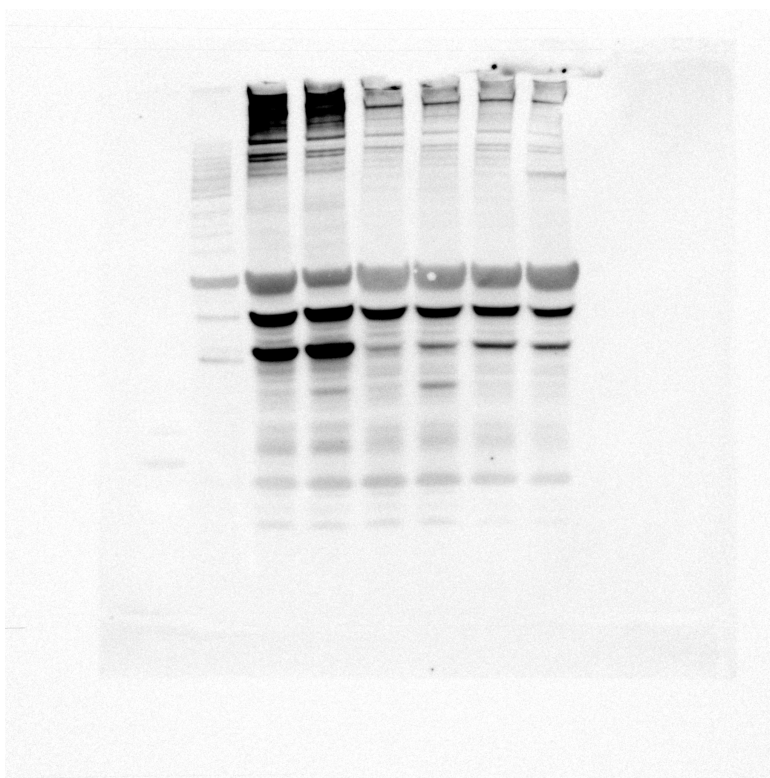
Figure 2J GSDMD
