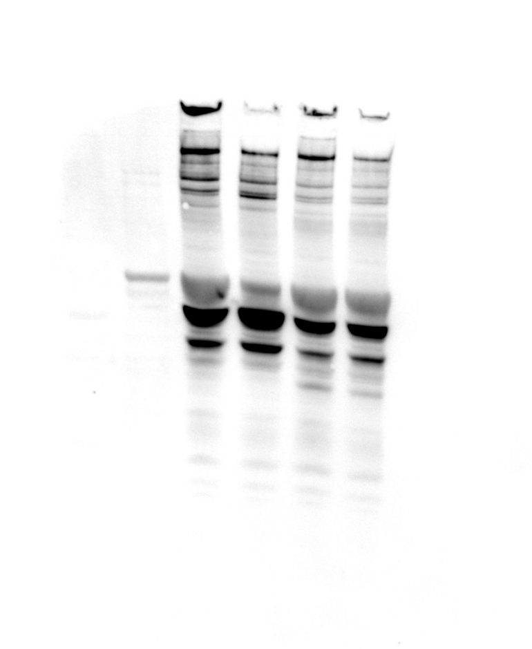
Figure 2J GSDMD
