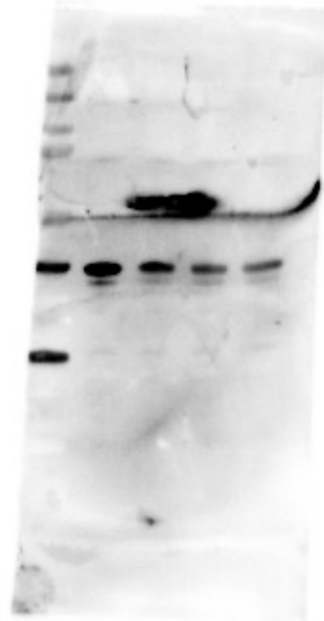
Figure 3A GAPDH
