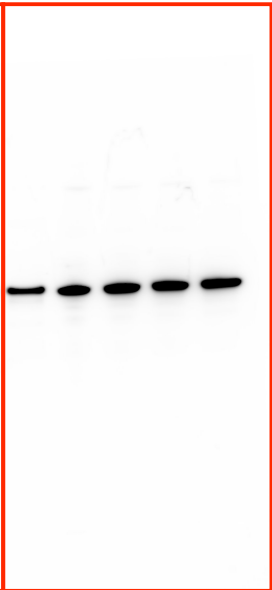
Figure 2J GAPDH
