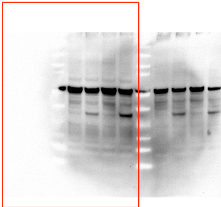
Figure 3A GSDMD
