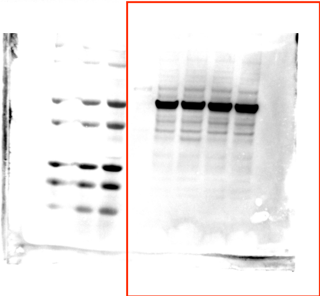
Figure 1B GSDMD
