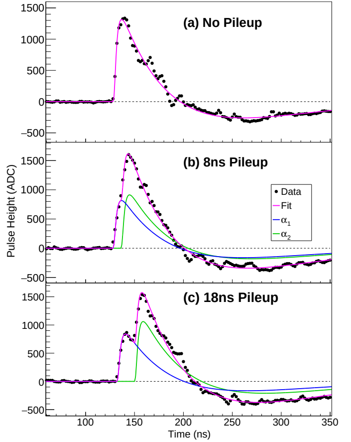
Fig. 6 Fits of a single peak (a), a pileup event with 8 ns time difference (b), and a pileup event with a 18 ns time difference (c). The pink curve is the total fit of the black experimental points, while the blue and green lines represent the decomposition in terms of the first and second decays, respectively.
