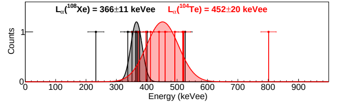
Fig. 7 Light yield measurements for the decay chain of ^{108}\text{Xe} (black) through ^{104}\text{Te} (red). Each point is marked with error from the resolution of the detector plus the error resulting from the trace deconvolution. Variations according to these errors are incorporated as the systematic errors.
