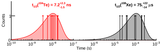
Fig. 2 Half-life measurements for ^{108}\text{Xe} (black) and ^{104}\text{Te} (red), extracted using the likelihood method described by Schmidt et al. [41]. The resulting half-life of ^{104}\text{Te} marks the fastest ground-state \alpha emission.
