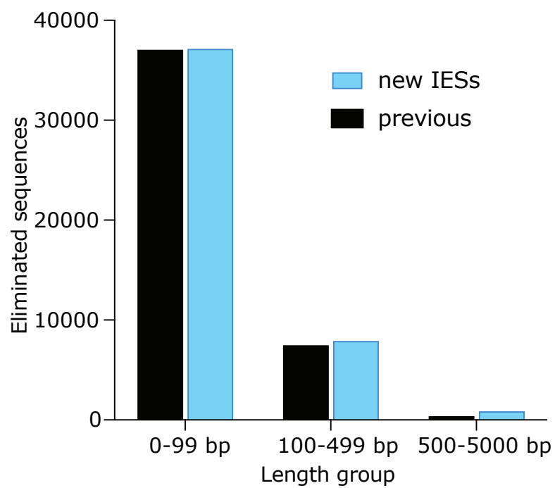
Supplementary Figure 3. The germline assembly reveals additional IESs
