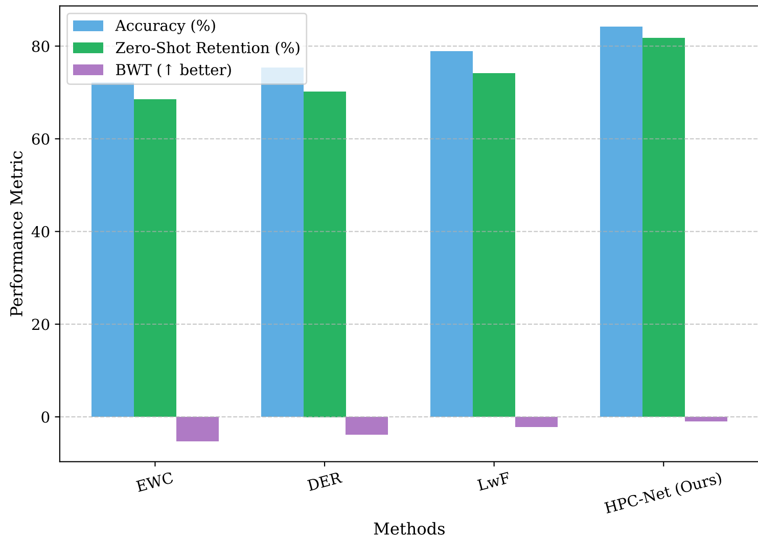
HPC-Net vs. Baselines
