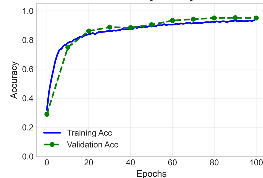
Accuracy History
