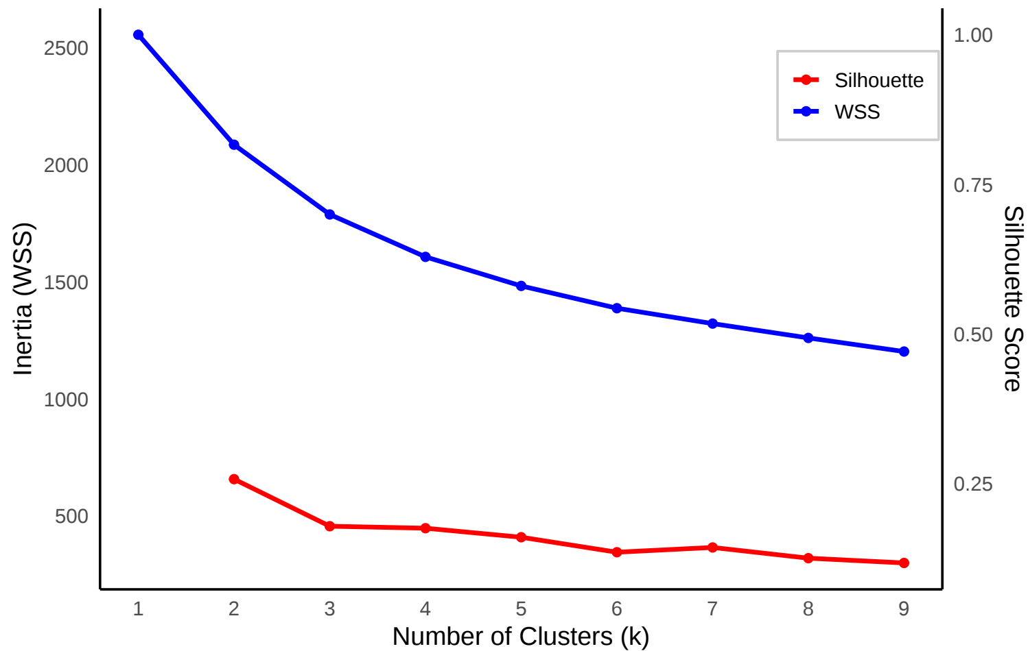
Elbow Method and Silhouette Score
