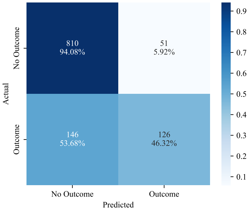
Confusion Matrix - Logistic
