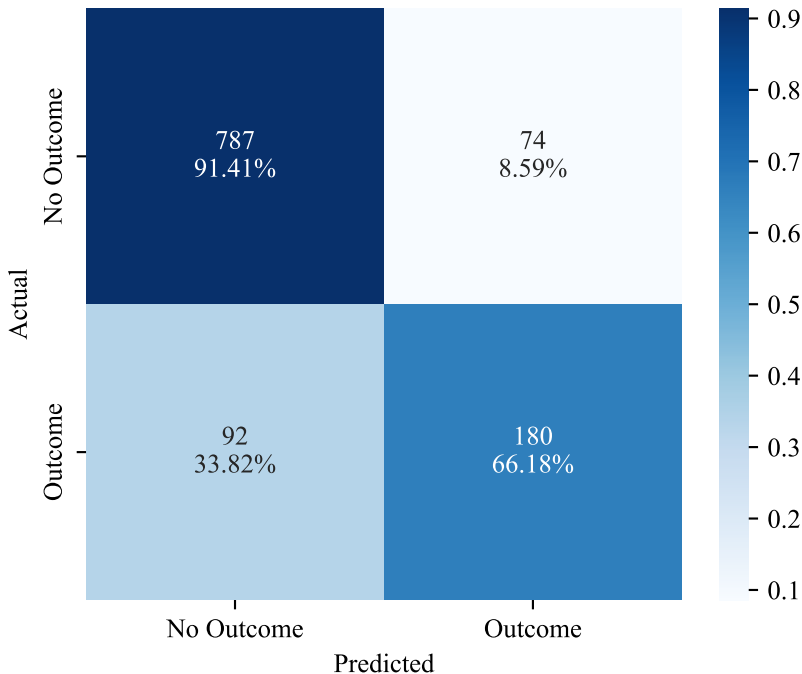
Confusion Matrix - DecisionTree
