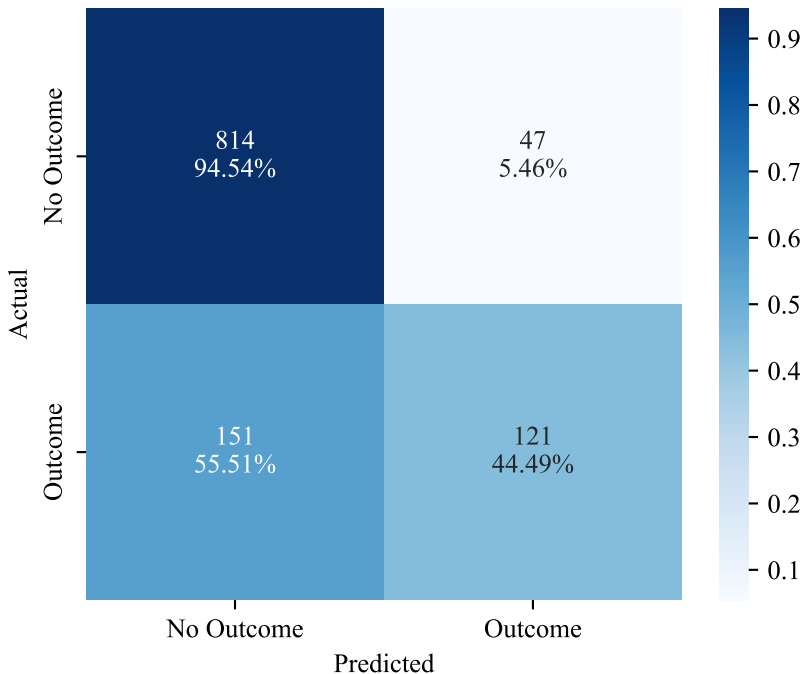
Confusion Matrix - SVM
