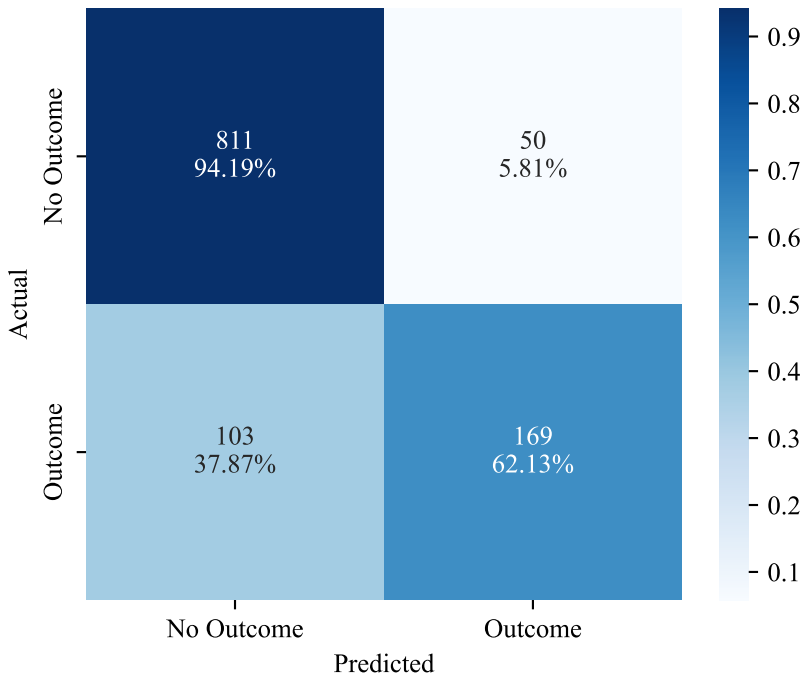
Confusion Matrix - ANN
