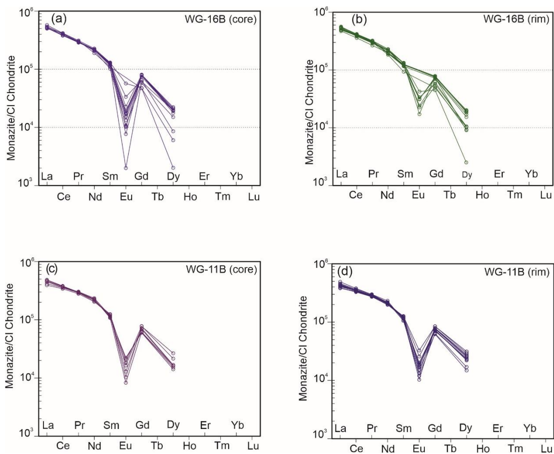
Supplementary figure 3 a-d CI chondrite normalized spider plot for monazite grains from the studied samples.
