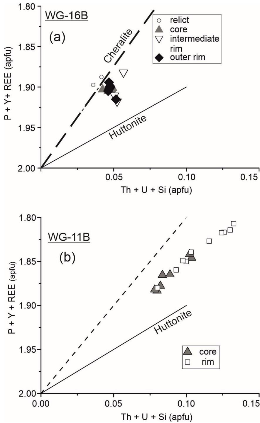
Supplementary figure 2 a, b P + Y + REE (apfu) versus Th + U + Si (apfu) plot for both the WG-16B and WG-11B samples.
