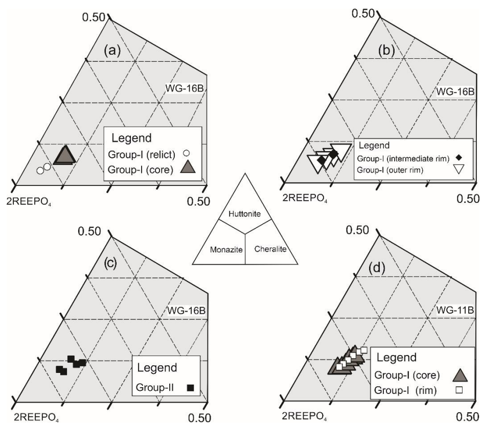
Supplementary figure 1 a-d Plot after (Linthout 2007) showing compositional variation among Monazite grains from the studied samples WG 16B and WG 11B.
