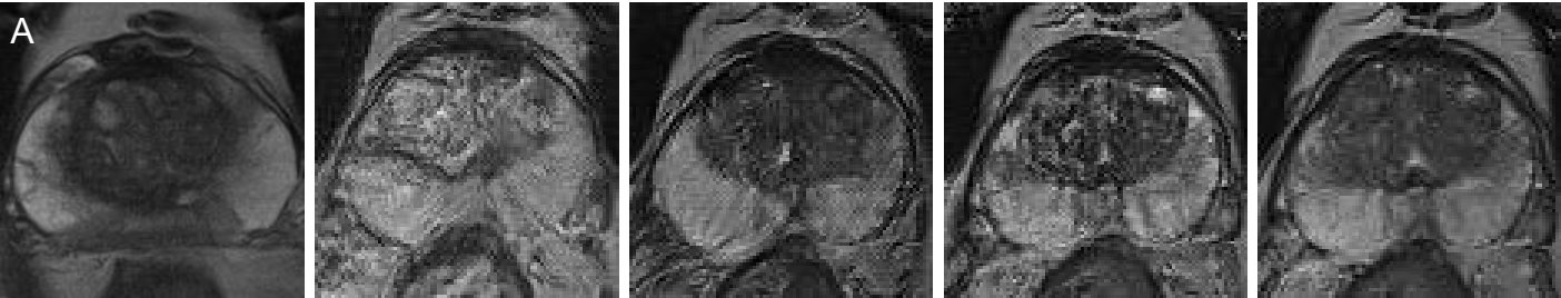
CycleGAN
