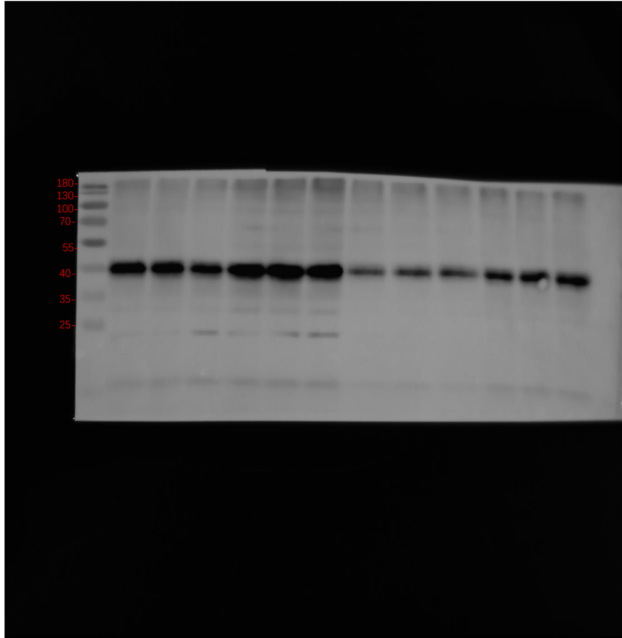
Figure7-Complex I
