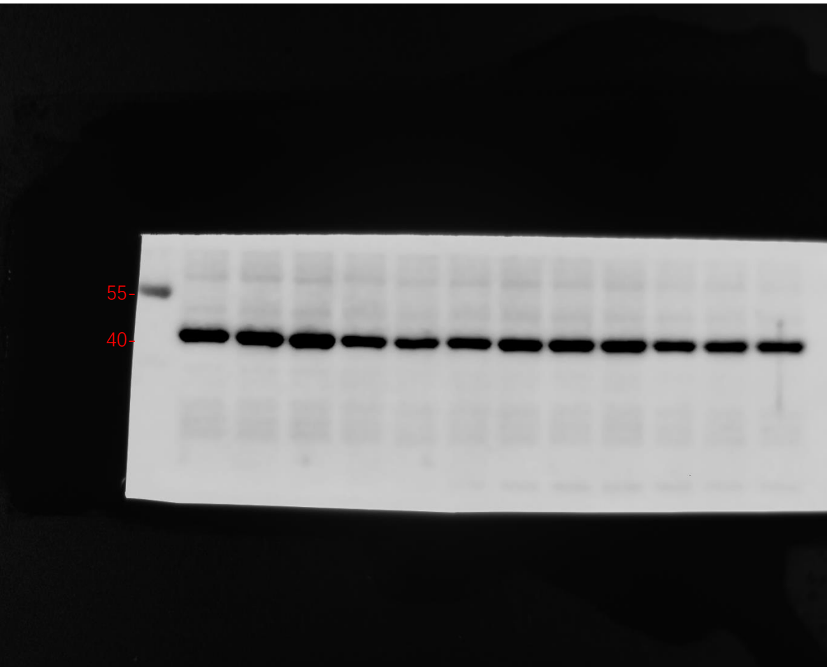
Figure 5- \beta -actin
