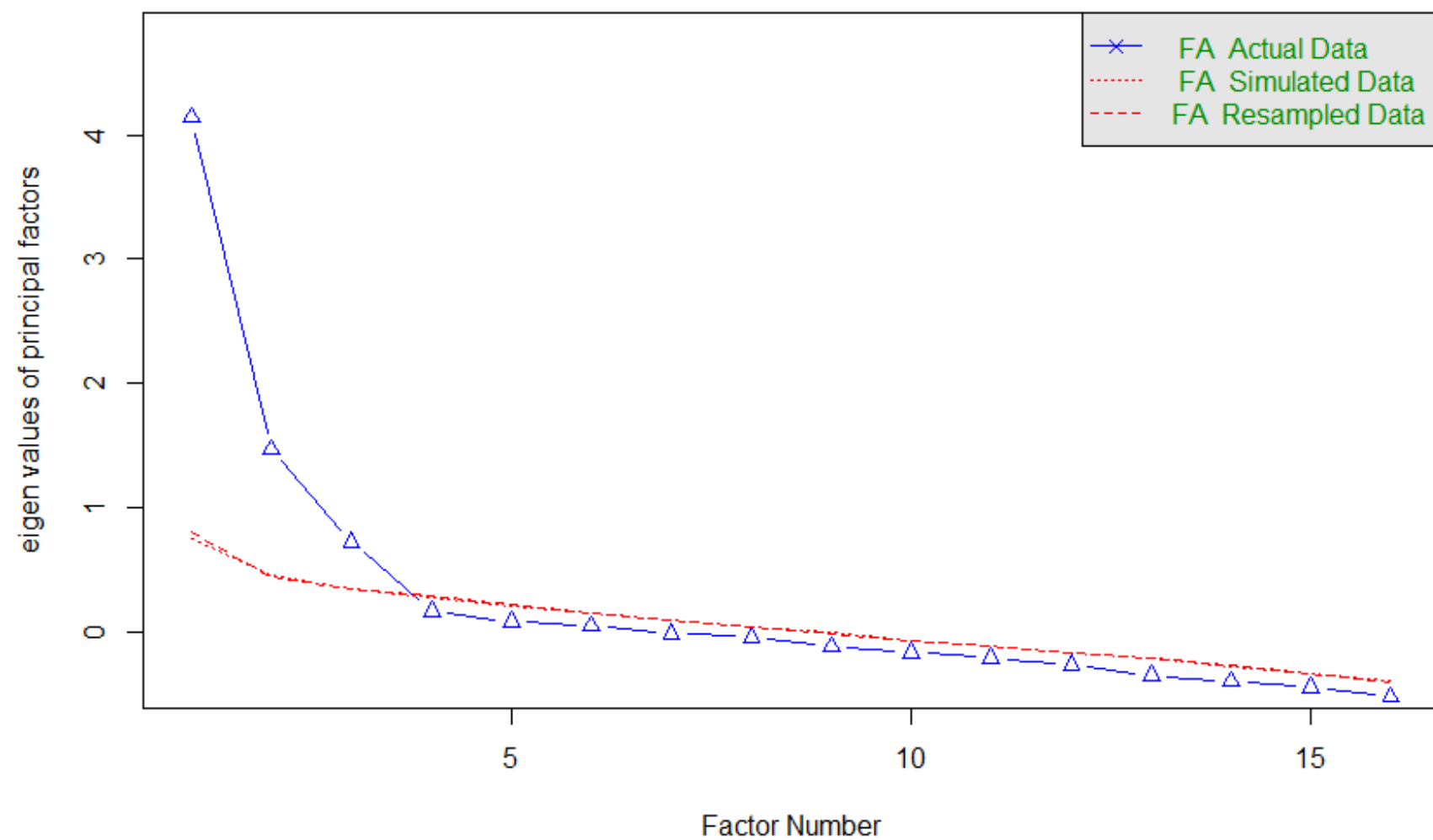
Parallel Analysis Scree Plots
