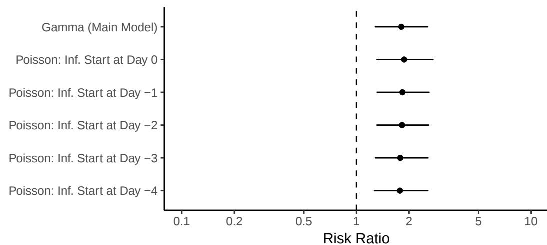
Infectiousness: A(H3N2) vs. A(H1N1)
