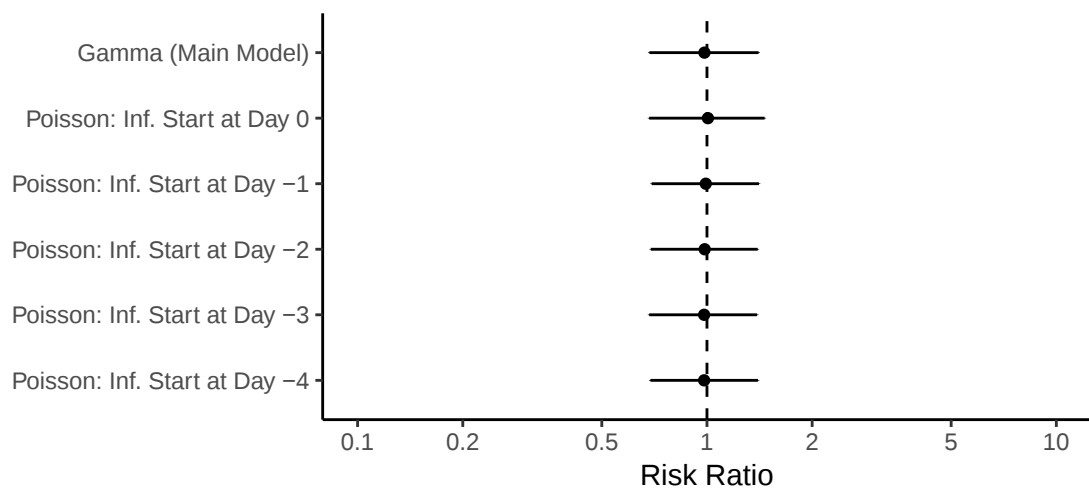
Infectiousness: Household Size >5 vs. Size 3
