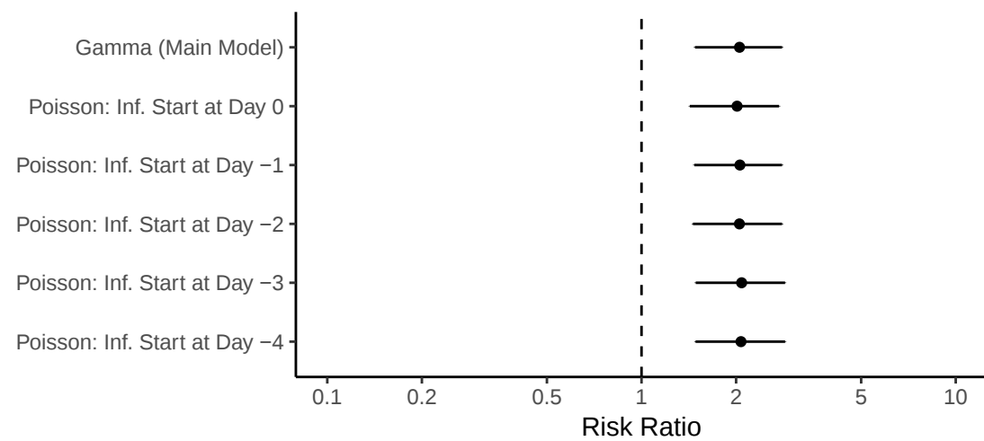
Infectiousness: Age < 6 vs. Adults
