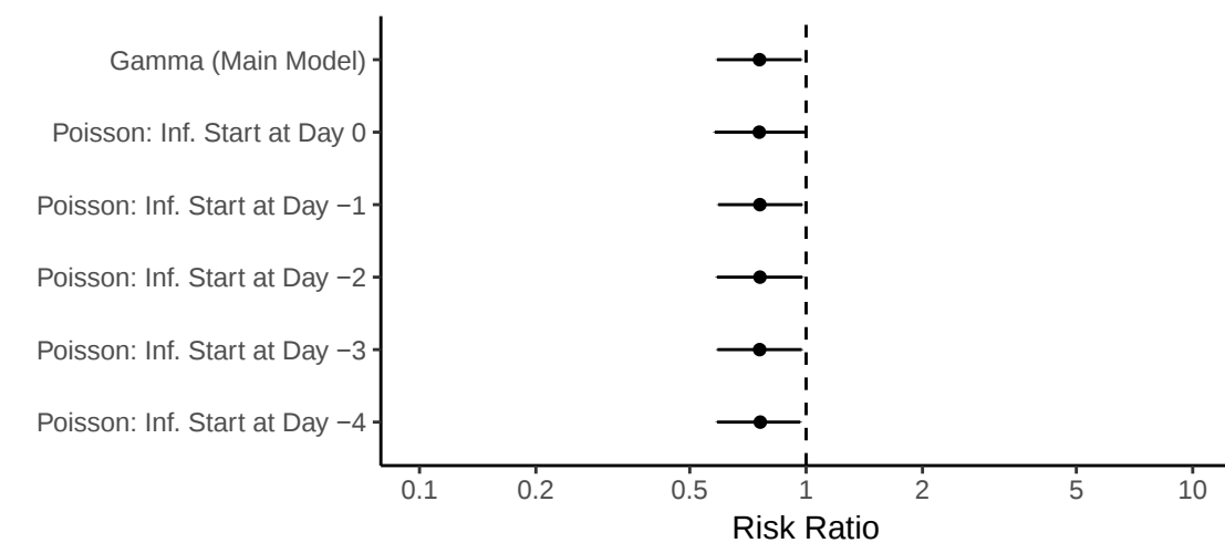
Infectiousness: Household Size 4 – 5 vs. Size 3
