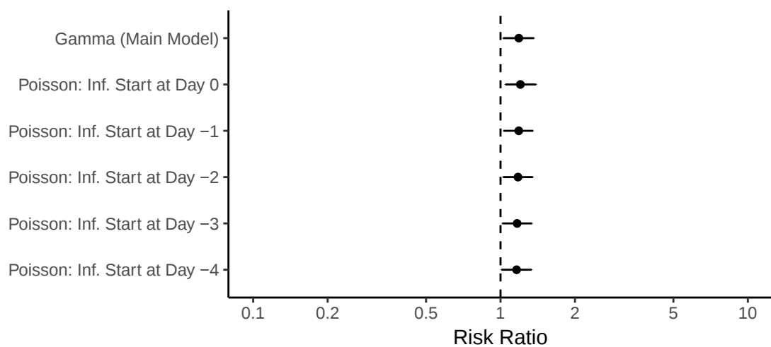
Infectiousness: A(H1N1)pdm vs. A(H1N1)
