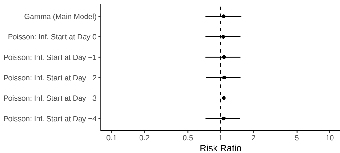
Infectiousness: Viral Load at Symptom Onset
