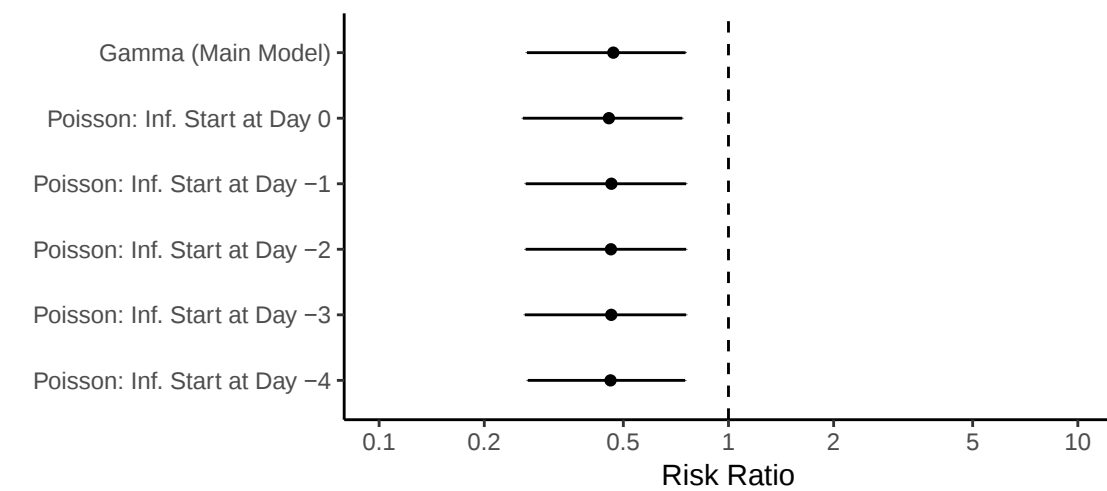
Infectiousness: Age 6 – 17 vs. Adults
