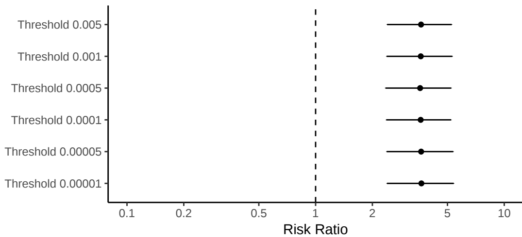
Susceptibility: Vaccination
