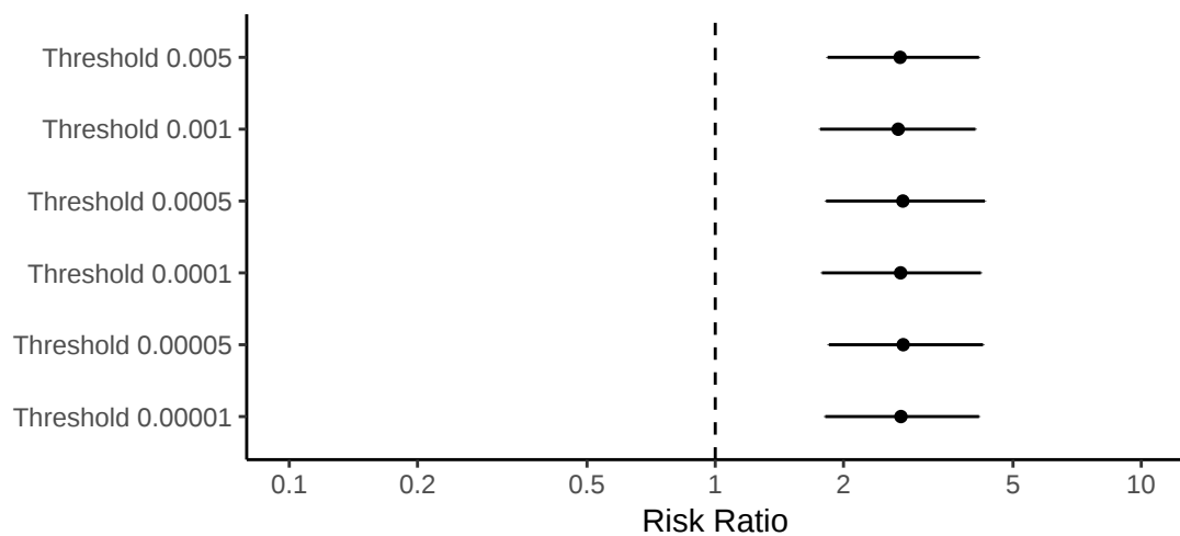
Infectiousness: Fever
