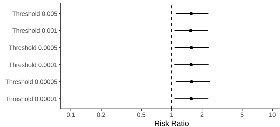
Infectiousness: Antiviral
