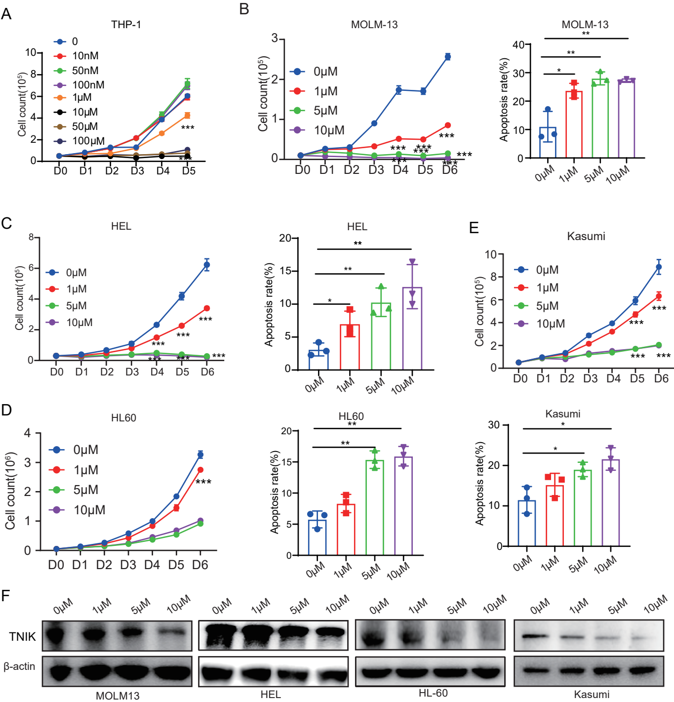
Supplemental Fig. 3 TNIK inhibition by TNIK-IN-1 suppresses AML proliferation
