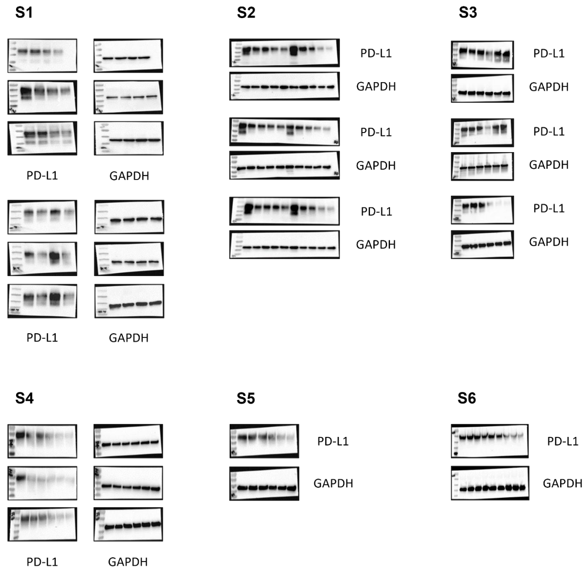
Supplementary Figure. This figure presents the original, uncropped Western blot images corresponding to the data shown in the main figures. The blots displayed in panels S1, S2, S3, S4, S5, and S6 correspond to those presented in Figure 1B–C, Figure 1E, Figure 1F, Figure 2C, Figure 5C, and Figure 6F, respectively.
