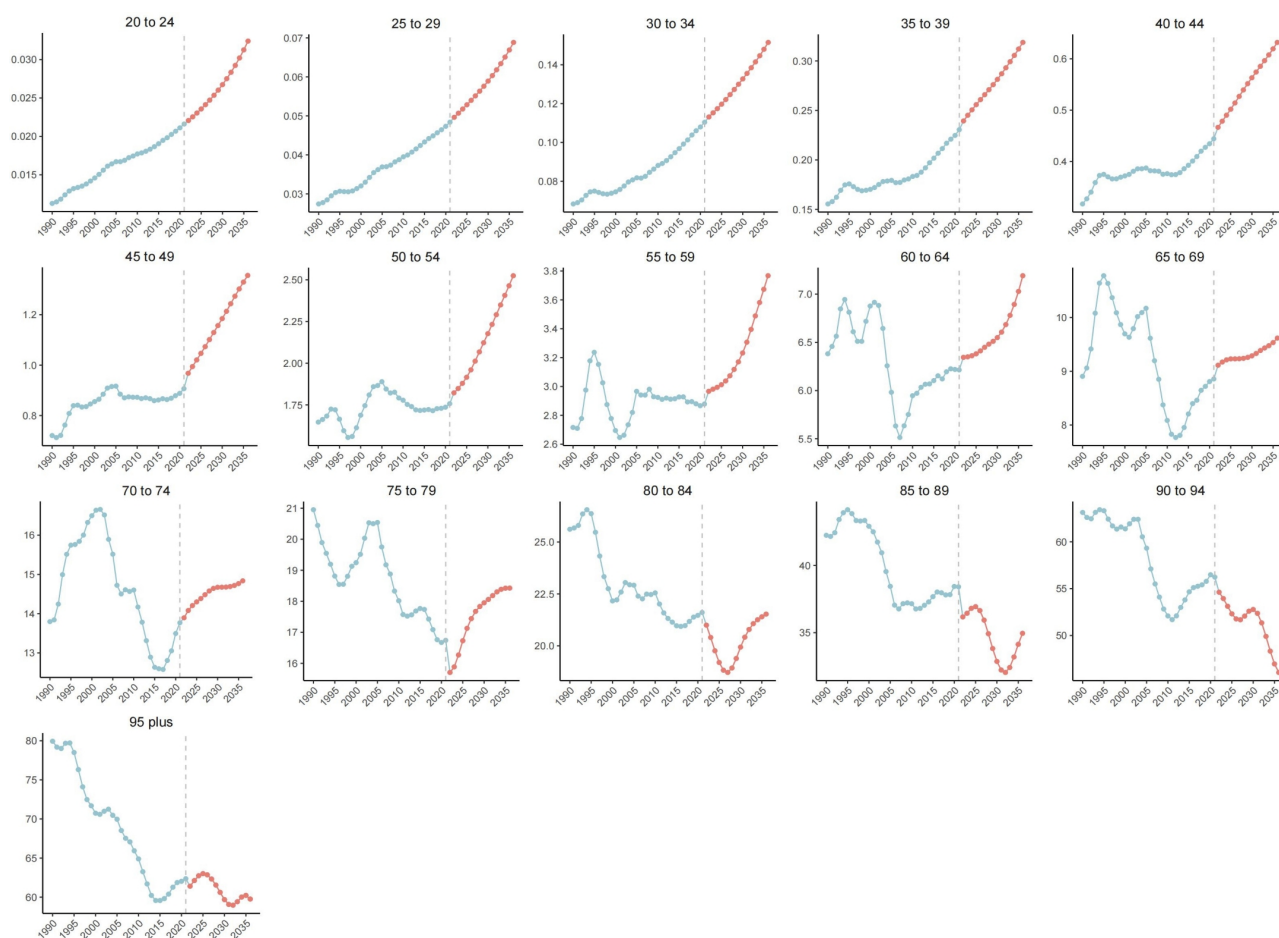
Supplementary Figure 6 Global predictions of death rates for different age groups of males between 2022 and 2036.
