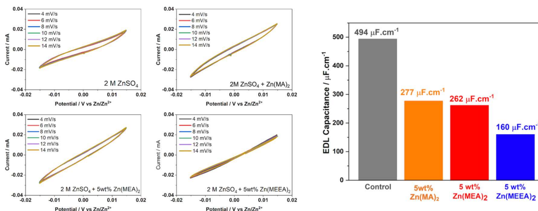
Fig. S12 – (left) \text{Zn} \parallel \text{Zn} symmetric cells at sweep rates of 4–14 mV/s within the non-Faradaic region ( \pm 15 \text{ mV} ) (right) EDLC was calculated using the equation: C = i_c / v of the different electrolytes
