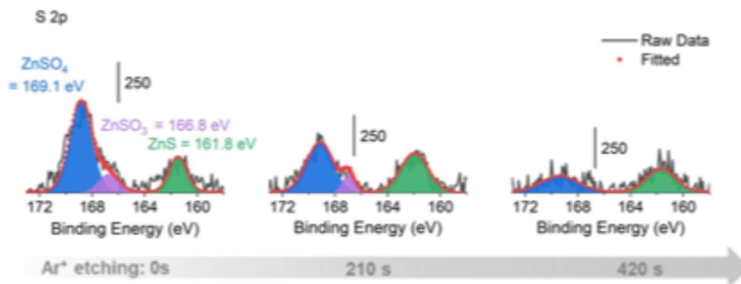
Fig. S21 – S 2p XPS spectra for Zn anodes cycled in 2 M ZnSO 4 + 10 M Urea + 5wt% Zn(MEEA) 2
