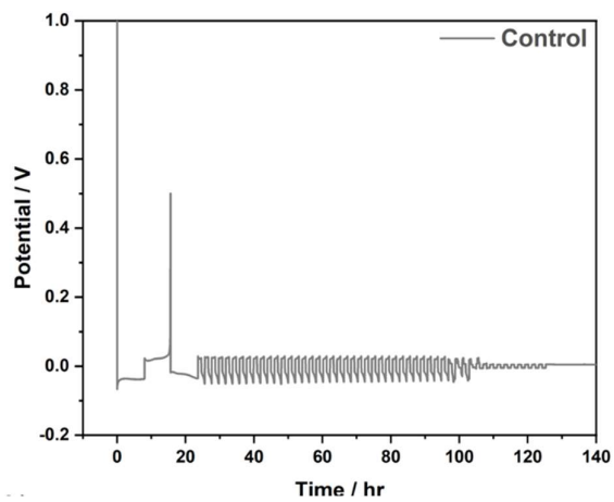
Fig. S10 – Zn || Cu cell cycled with 2 M ZnSO 4 using CE% method following Xu et al. which failed
