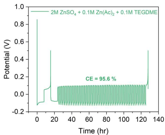
Fig. S15 - CE% determination with 2 M ZnSO 4 + 0.1M Zn(Ac) 2 + 0.1M TEGDME in Zn || Cu.
