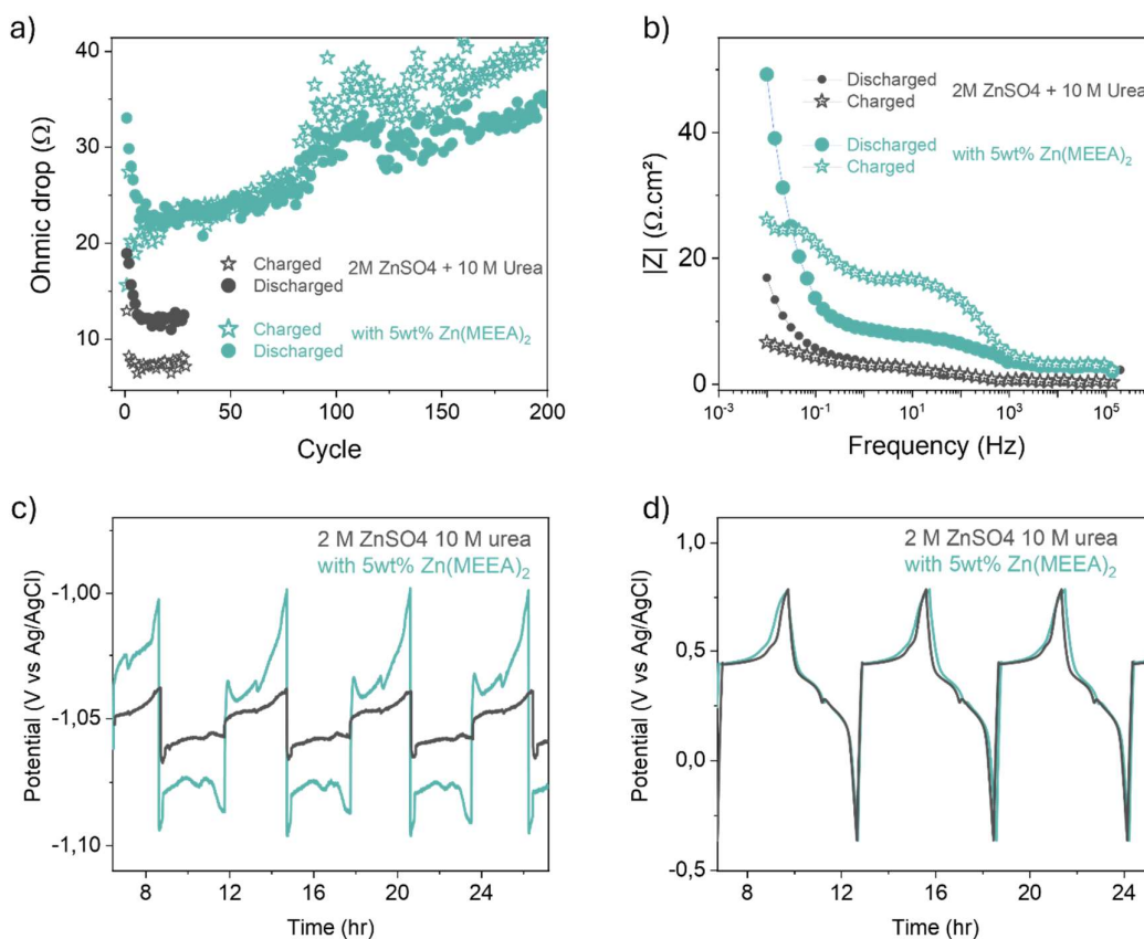
Fig. S22 - (a) Ohmic drop of the full cell shown in Fig. 6b after charge and discharge states. (b) Electrochemical impedance of the Zn anode measured in a three-electrode configuration, with and without Zn(MEEA) 2 . (c) Potential of the zinc foil (reference/counter electrode) during galvanostatic cycling in Zn/MnO 2 three-electrode cells, with and without Zn(MEEA) 2 . (d) Potential vs. time of the MnO 2 working electrode with and without Zn(MEEA) 2 additives.
