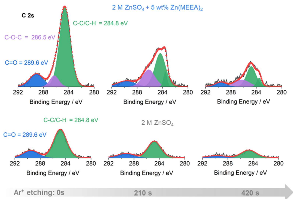
Fig. S18 – C 2s XPS spectra for Zn anodes cycled in 2 M \text{ZnSO}_4 + 5wt% \text{Zn(MEEA)}_2 (top) and 2 M \text{ZnSO}_4 (bottom) with \text{Ar}^+ ion beam up to a depth of \sim 10 nm.
