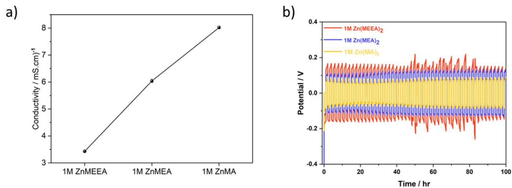
Fig. S8 – a) Ionic conductivity for Zn(MA) 2 , Zn(MEA) 2 and Zn(MEEA) 2 and b) Zn || Zn symmetric cells for 1 M Zn(MA) 2 (orange), 1 M Zn(MEA) 2 (blue) and 1 M Zn(MEEA) 2 (red).
