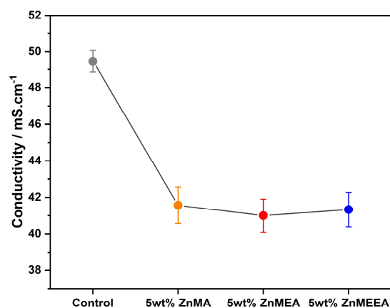
Fig. S9 – Ionic conductivity for 2M ZnSO 4 , 5wt% Zn(MA) 2 , Zn(MEA) 2 and Zn(MEEA) 2 in 2M ZnSO 4
