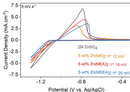
Fig. S11 – Cyclic voltammetry (CV) of 2 M \text{ZnSO}_4 (grey), 2 M \text{ZnSO}_4 + 5wt% \text{Zn(MA)}_2 (orange), 2 M \text{ZnSO}_4 + 5wt% \text{Zn(MEA)}_2 (red) and 2 M \text{ZnSO}_4 + 5wt% \text{Zn(MEEA)}_2 (blue) on a glassy carbon electrode at a scan rate of 5 \text{ mV.s}^{-1}
