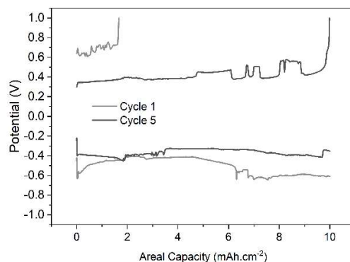
Fig. S13 – \text{Zn} \parallel \text{Cu} cell cycled with 2 M \text{ZnSO}_4 at 5 \text{ mA.cm}^{-2} / 10 \text{ mAh.cm}^{-2}
