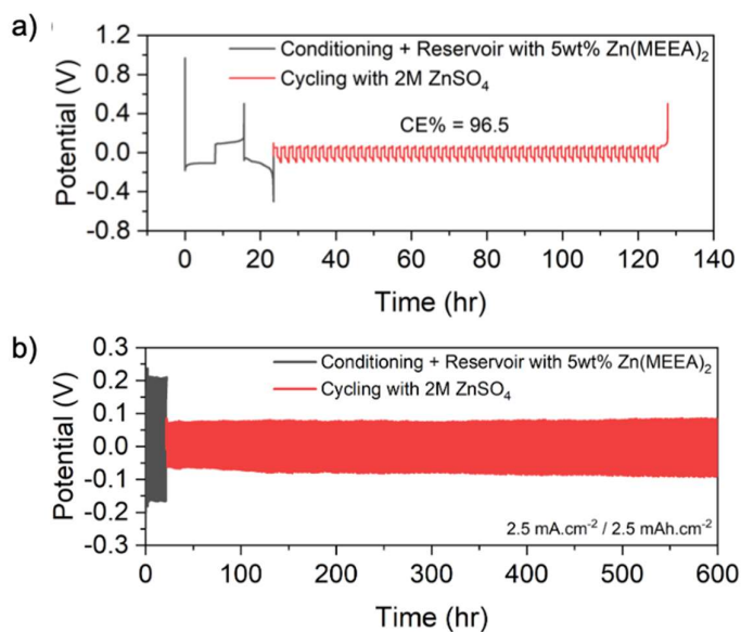
Fig. S19 – a) CE% determination with electrodes first conditioned with 2 M \text{ZnSO}_4 + 5wt% \text{Zn(MEEA)}_2 and then cycled with 2 M \text{ZnSO}_4 in \text{Zn} \parallel \text{Cu} & b) \text{Zn} \parallel \text{Zn} cells with electrodes first conditioned with 2 M \text{ZnSO}_4 + 5wt% \text{Zn(MEEA)}_2 and then cycled with 2 M \text{ZnSO}_4 .
