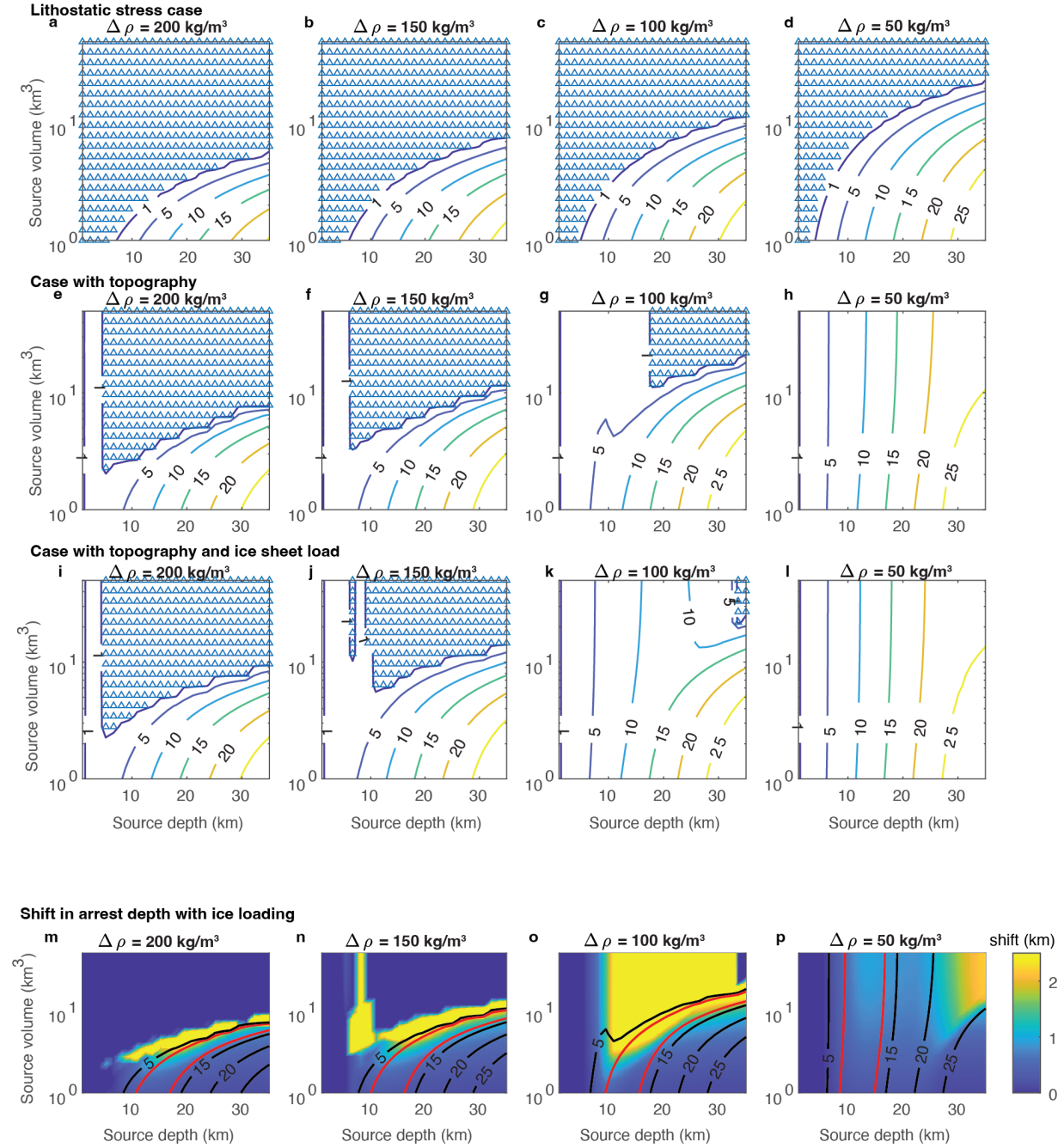
Fig. S6: Dike model results for critical overpressure of 10 MPa
