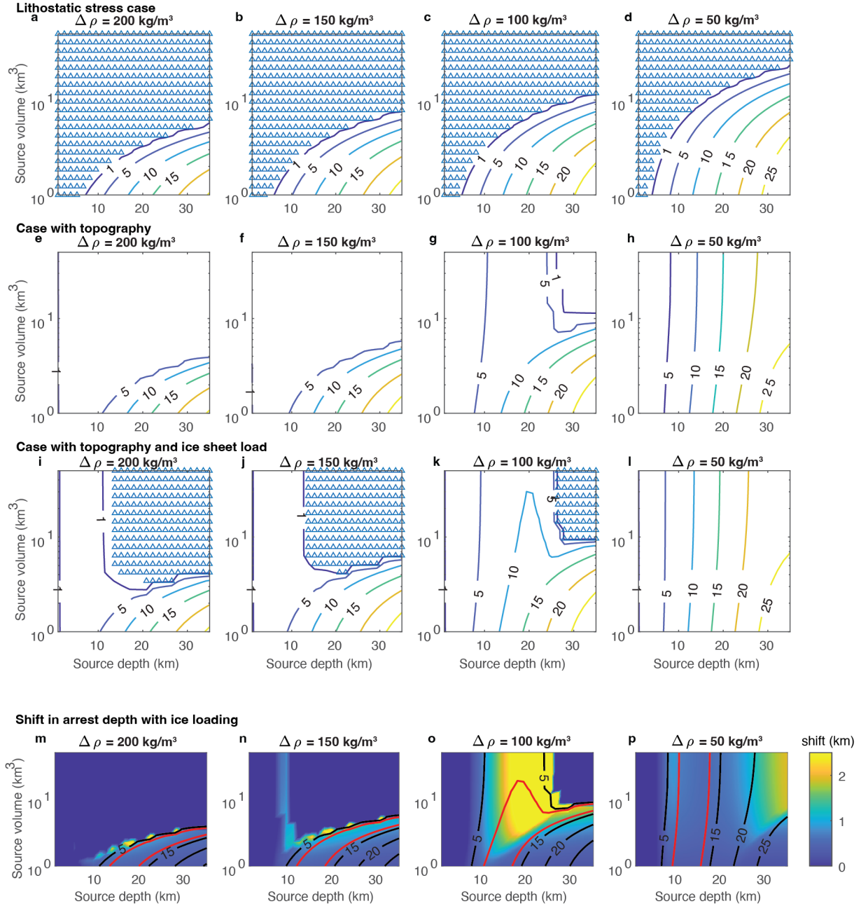
a-l , Dike arrest depths in km below msl shown as colored and labeled contours, plotted as a function of source depth and source volume for different crust-magma density contrasts ( \Delta\rho ). Dikes that erupt are shown as open blue triangles. m-p , Shift in dike arrest depth in km (positive downward) shown in blue-to-yellow colors as a function of source depth and source volume. Black curves are contours of arrest depths (in km) under ice-free conditions, with red lines representing storage depths at Mocho-Choshuenco (7-13 km) during the pre-LGM period. Parameters used: dike strike = N63, \mu = 10 GPa, r = 1.5 m, \Delta P_{crit} = 20 MPa.
