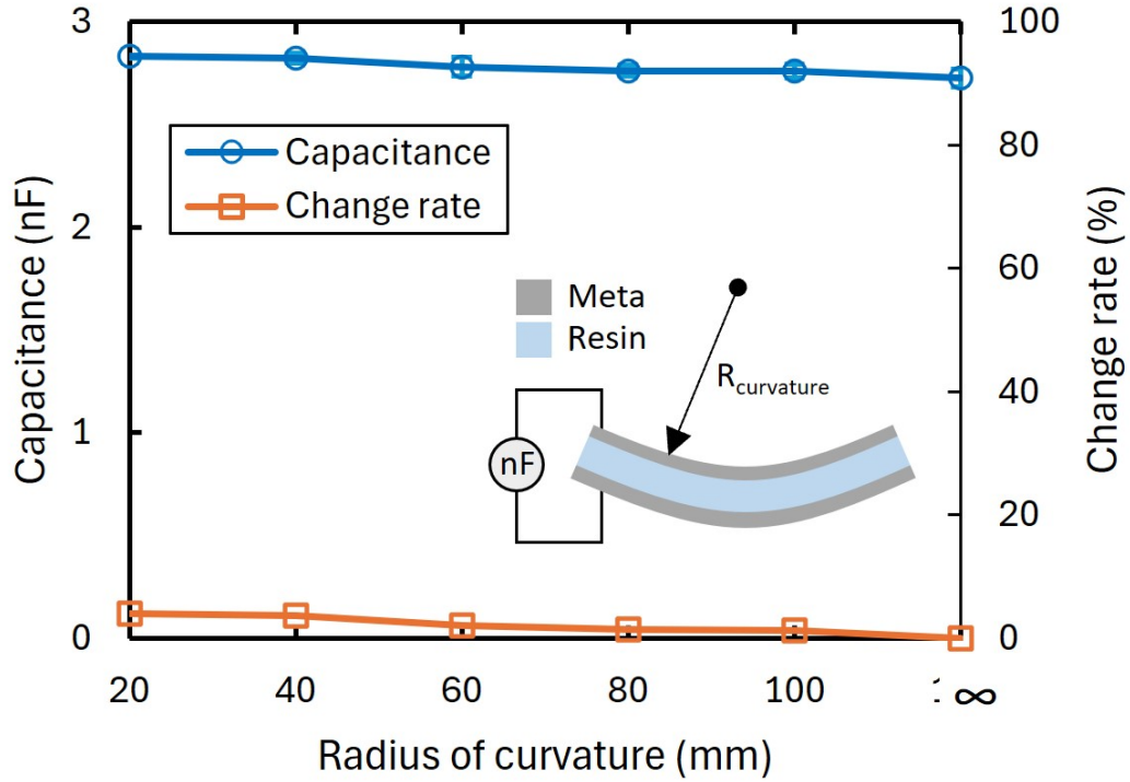
Figure S 1: Measured capacitance values of the flexible electrovibration layer under the varying radii of curvature.
