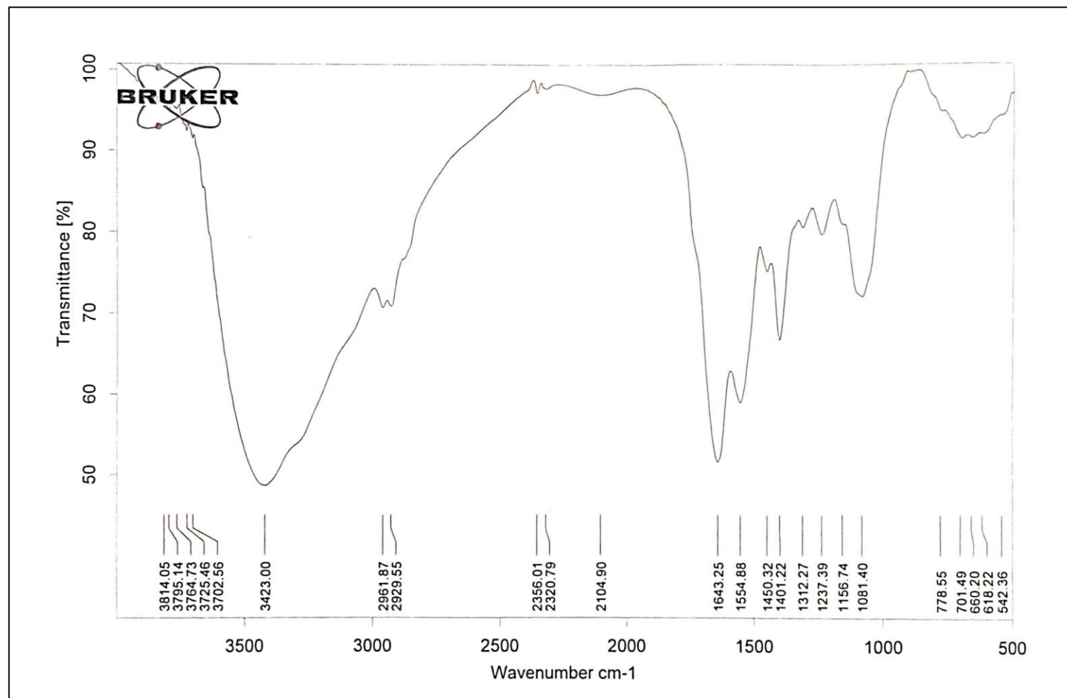
Fig. S4 IR spectra of TNCB-27 with no treatment
