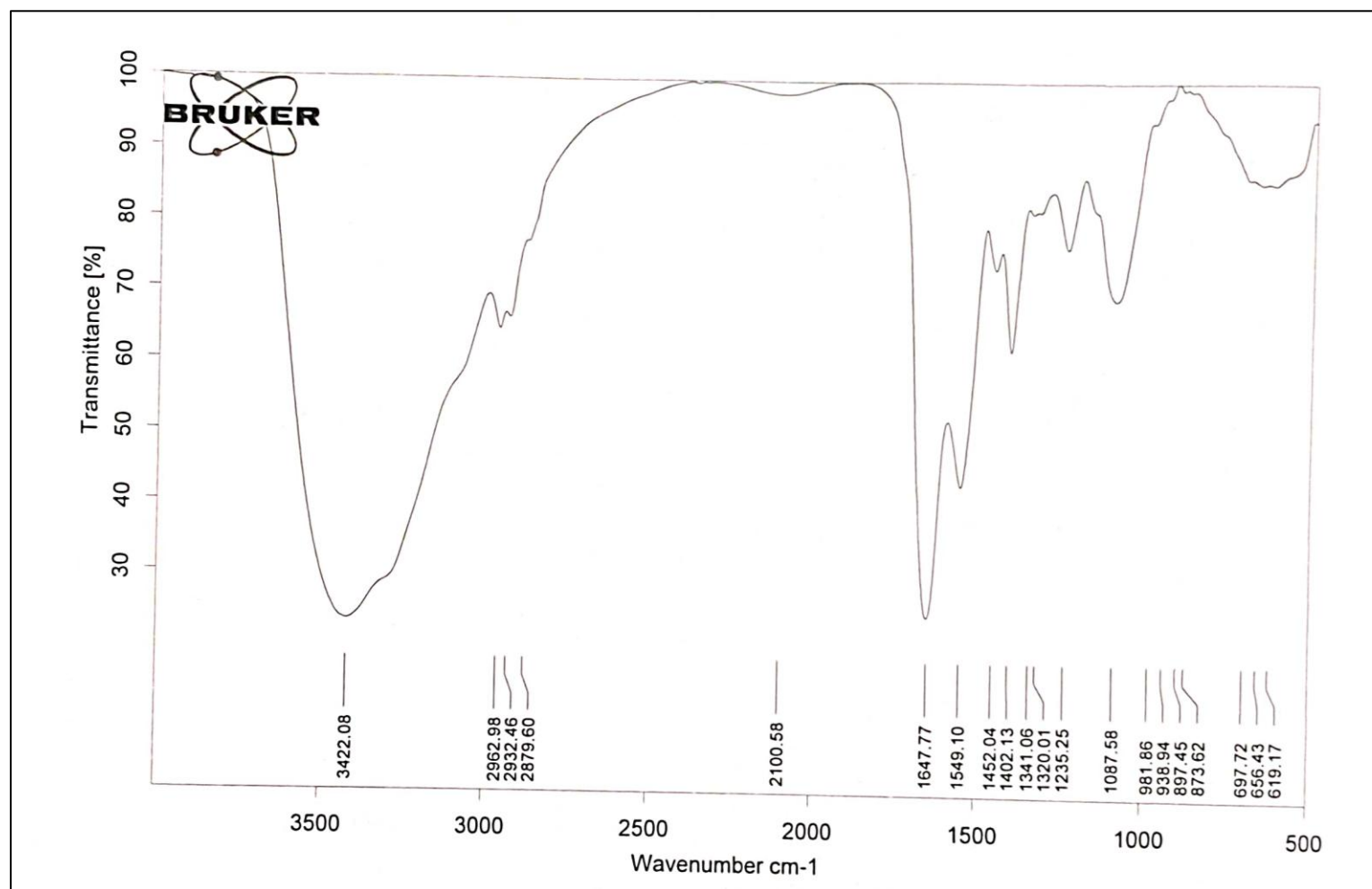
Fig. S3 IR spectra of TNB-16 with As 5+ treatment
