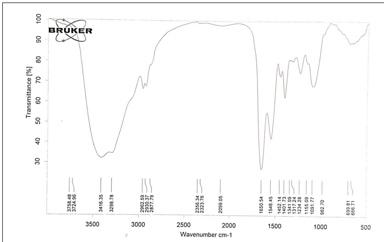
Fig. S2 IR spectra of TNB-16 with As 3+ treatment
