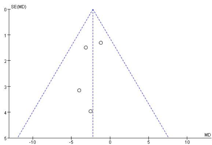
Funnel Plots for eWMT on Rumination
