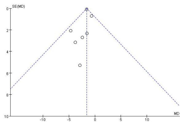
Funnel Plots for eWMT on depression
