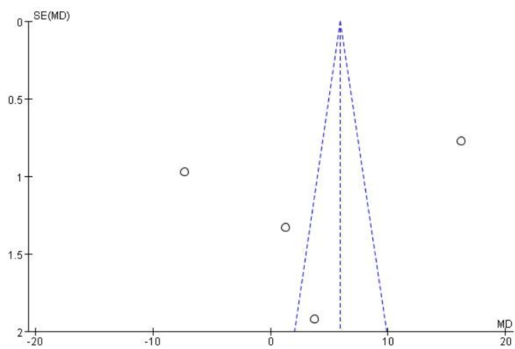
Funnel Plots for eWMT on Reappraisal
