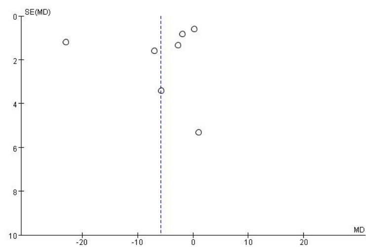
Funnel Plots for eWMT on working memory capacity
