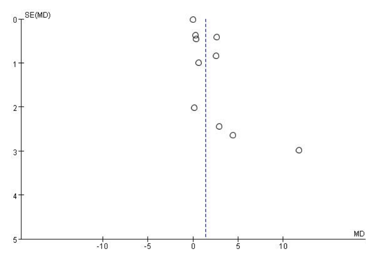
Funnel Plots for eWMT on working memory capacity
