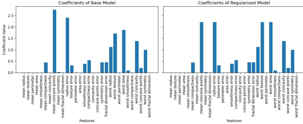
Figure 3: Coefficients of logistic regression models before and after S_3 regularisation.
