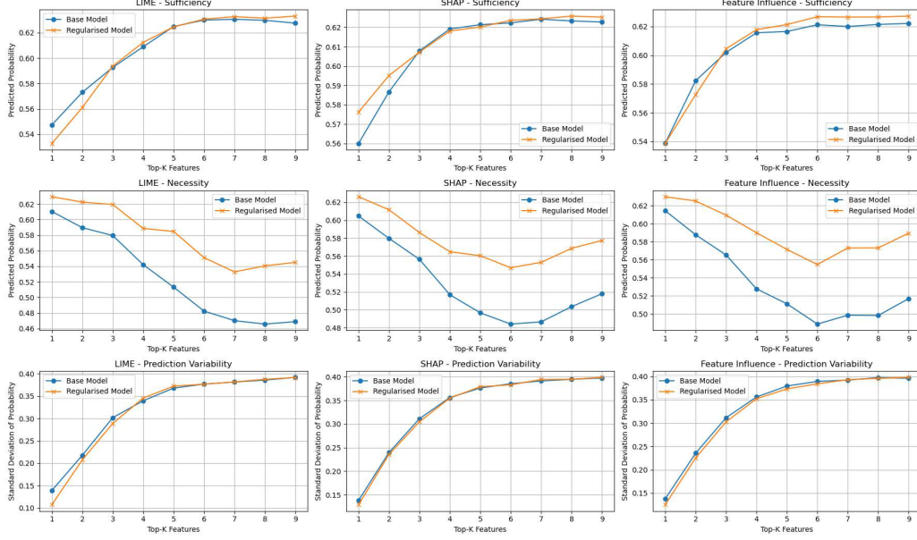
Figure 4: Comparison of explanation metrics across models and explanation methods. Rows correspond to sufficiency (top), necessity (middle), and prediction variability (bottom). Columns represent LIME, SHAP, and feature influence methods. Each plot shows results for the base model (blue) and the regularised model (orange) across different numbers of top-K features.
