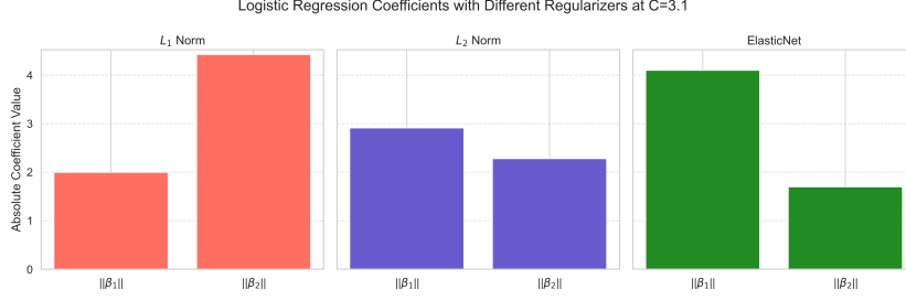
Figure 2: Logistic regression coefficients for different regularizers ( L_1 , L_2 , ElasticNet) on the same dataset, with regularisation strength set to C = 3.1 .
