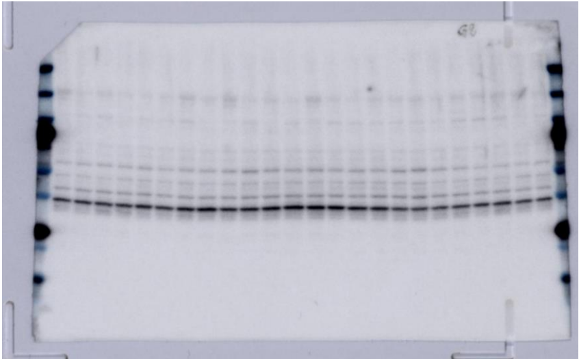
GAPDH
