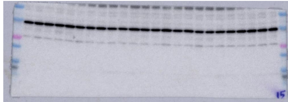
GAPDH
