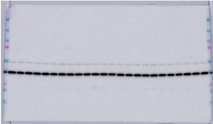
GAPDH
