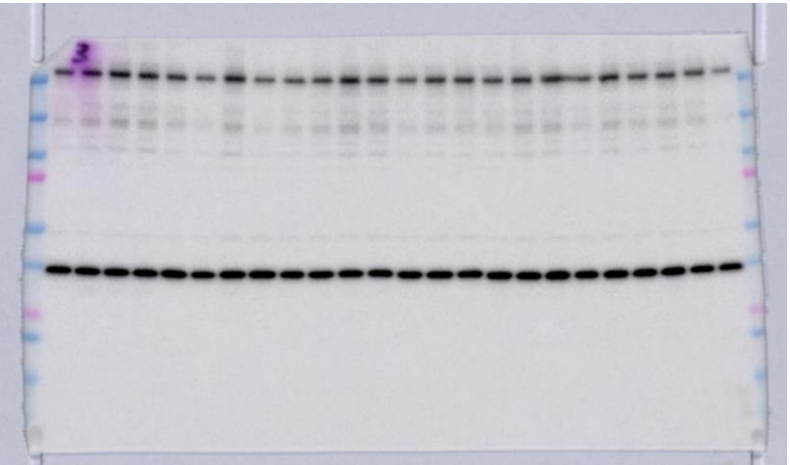
GAPDH
