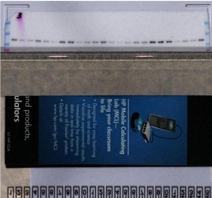
SCAP
