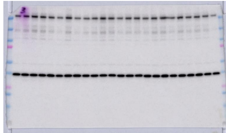
GAPDH
