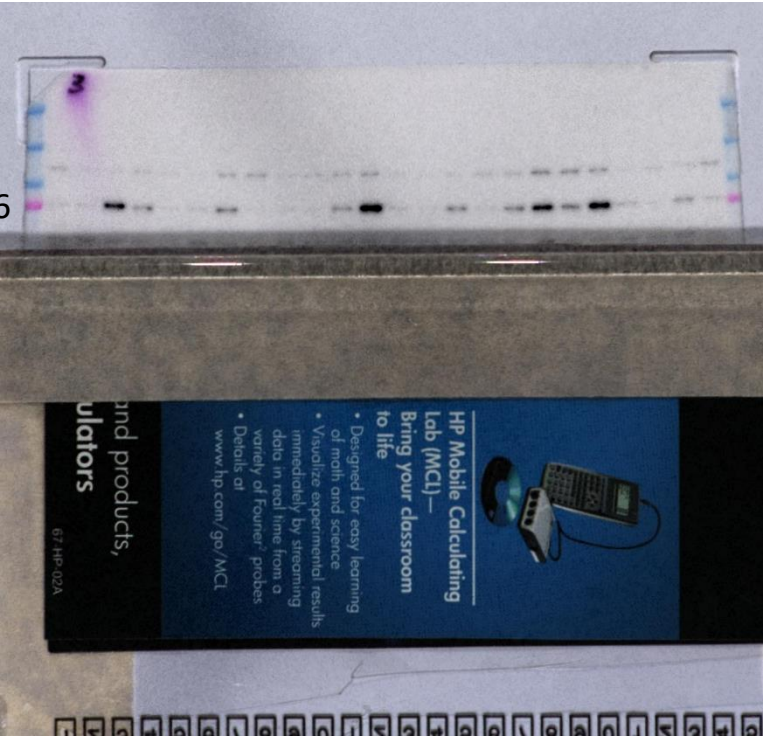
CD36
