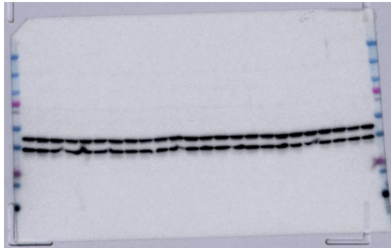
ACTIN
