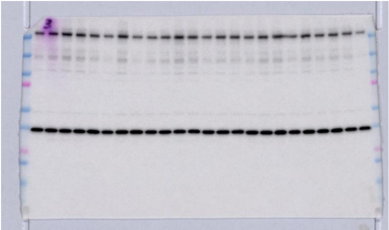
GAPDH
