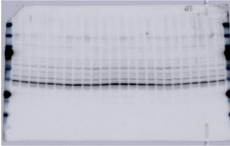
GAPDH
