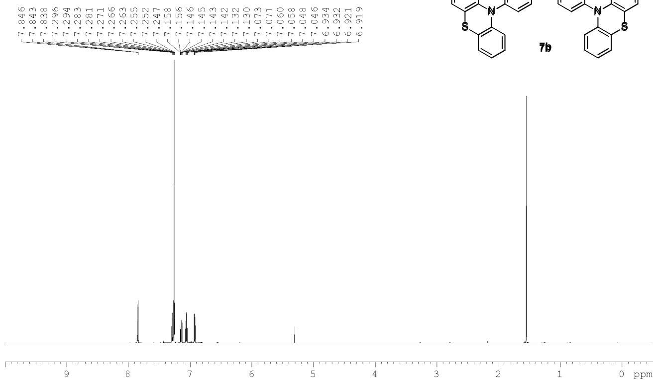
^1\text{H} NMR (600 MHz) spectrum of 7b ( \text{CDCl}_3 )
