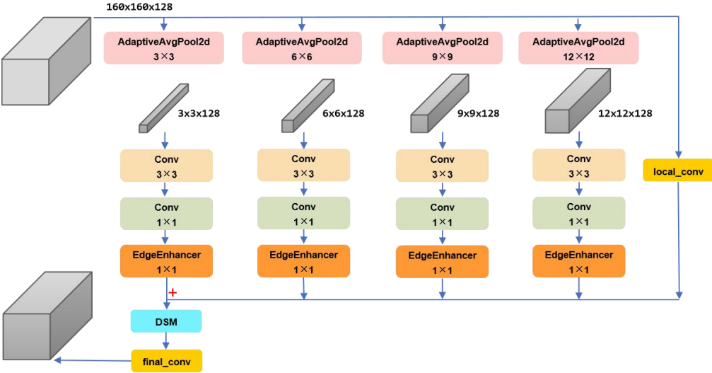
Fig. 8 Multi-scale Edge Information Extraction module
