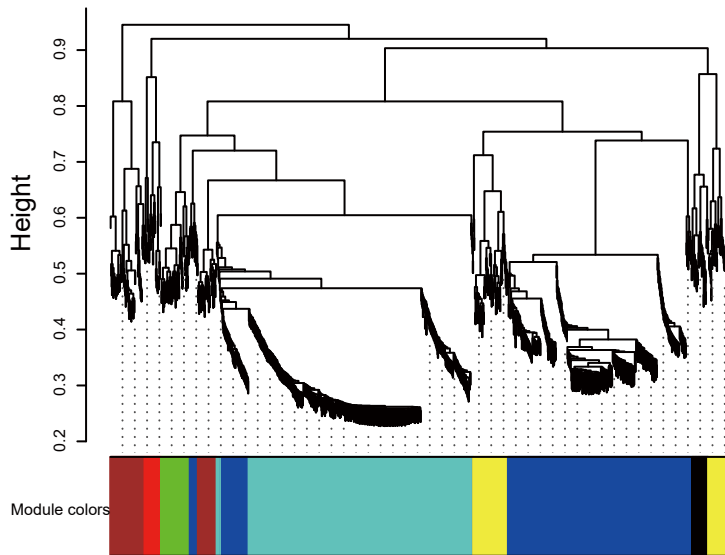
Cluster Dendrogram
