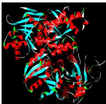
3KS9
