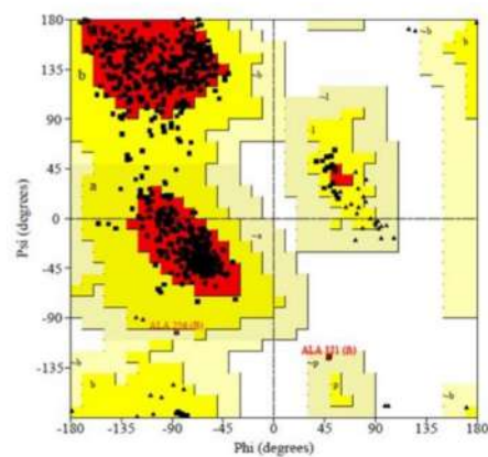
RAMACHANDRAN PLOT
