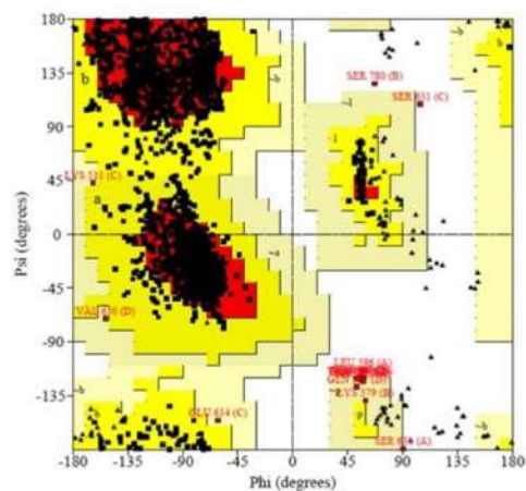
RAMACHANDRAN PLOT
