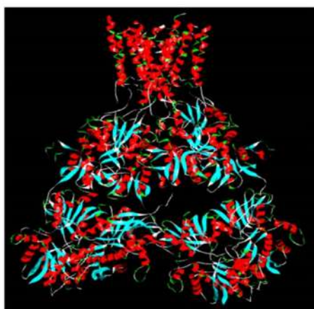
5L1G
