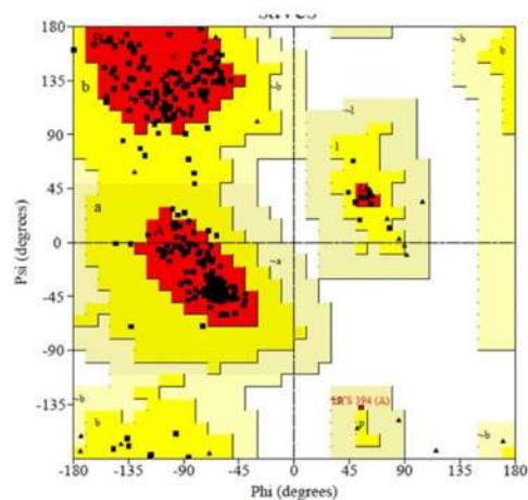
RAMACHANDRAN PLOT
