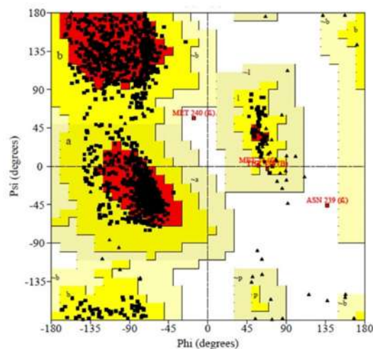
RAMACHANDRAN PLOT
