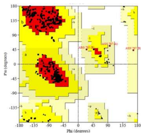
RAMACHANDRAN PLOT
