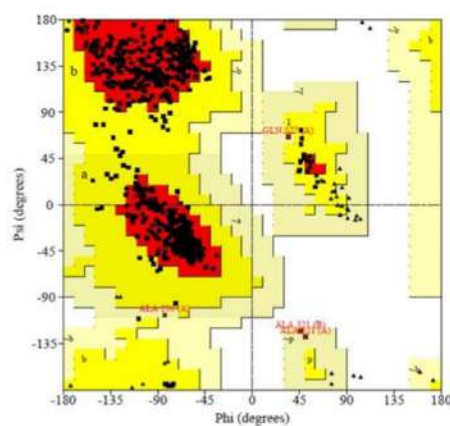
RAMACHANDRAN PLOT
