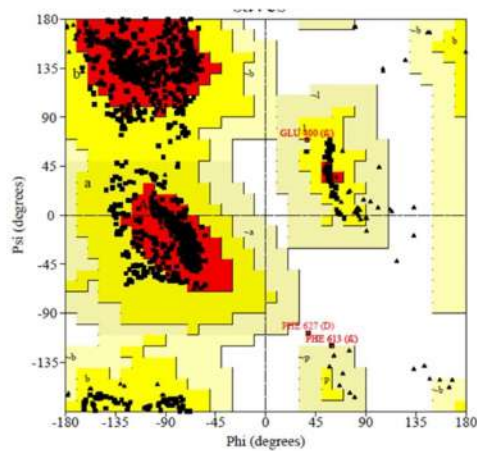
RAMACHANDRAN PLOT
