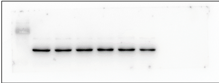
Fig C-p62
