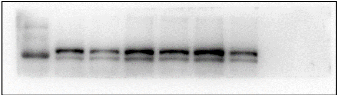
Fig J-FSHR
