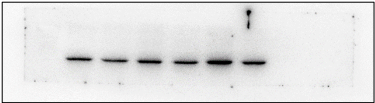
Fig L-3β-HSD
