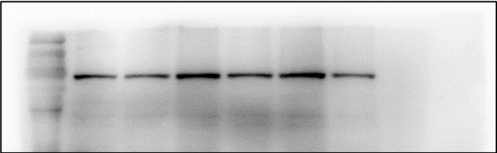
Fig J-FSHR
