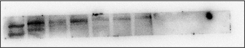
Fig G-mTOR
