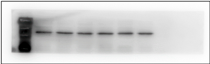
Fig K-α-Tublin
