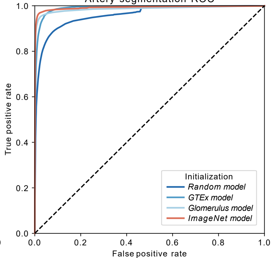
Vessel model Artery segmentation ROC
