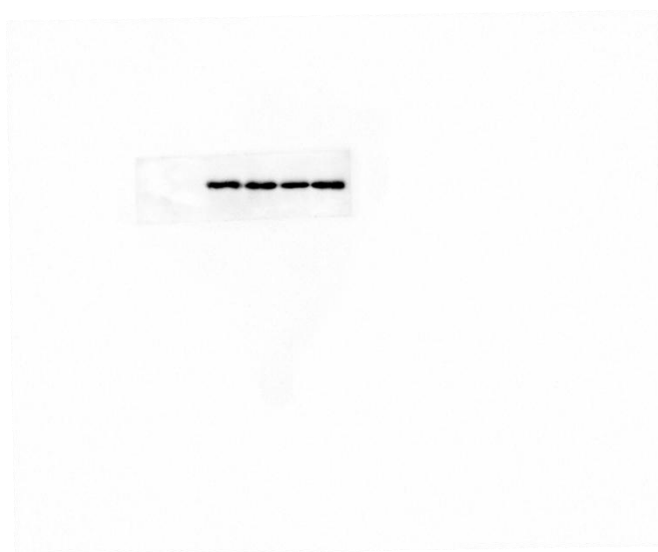
ITGB4-H1299
