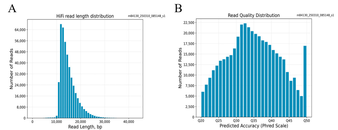
Figure S1 | HiFi Read Statistics for O. vulgare Mitogenome Sequencing. (A) Distribution of HiFi read lengths. (B) Distribution of predicted read quality (Q score) across HiFi reads.
