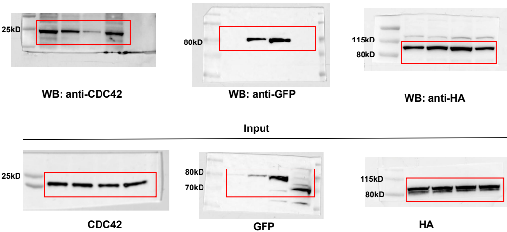
IP: anti-HA
