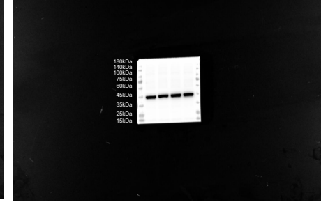
\beta -actin
