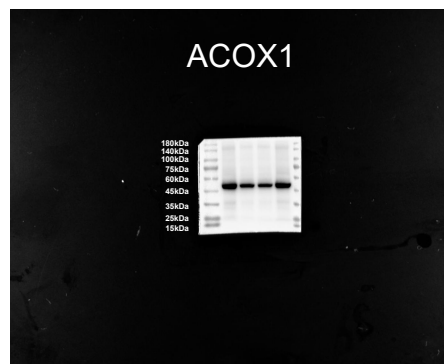
MCF-7
