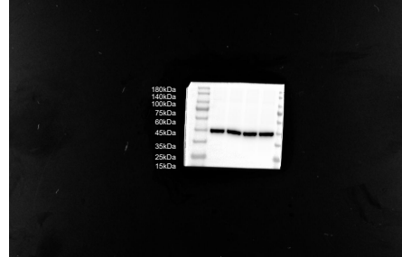
\beta -actin
