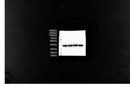
\beta -actin
