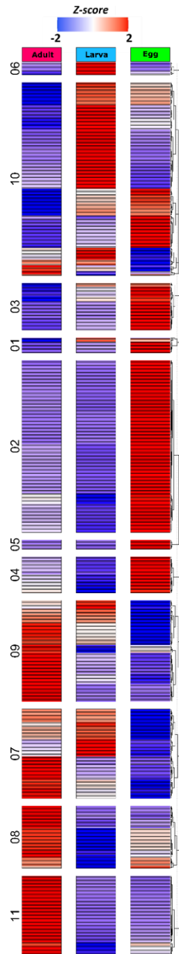
Supplementary Figure 2. Heatmap of all quantifiable proteins across BSF developmental stages. Protein abundance values (Z-score) are shown for adult, larva, and egg samples. Proteins were grouped into clusters using hierarchical clustering based on their expression profiles across all stages.
