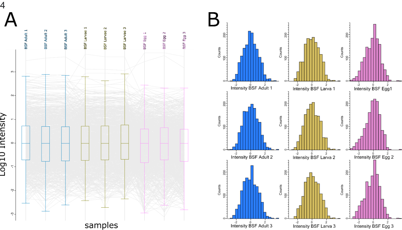
5 Supplementary Figure 1. Exploratory analysis and quality assessment of proteomic 6 data. (A) Boxplots of normalized \log_{10} intensity values across all BSF samples, illustrating 7 sample distribution and variability. (B) Histograms showing the distribution of protein \log_{10} 8 intensities (X-axis) and corresponding protein counts (Y-axis) for each biological replicate per 9 developmental stage.
