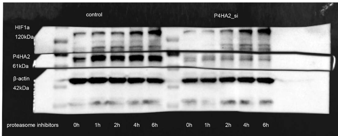
Fig.6I Western blot results of HIF-1 \alpha protein expression in SiHa and CasKi cells treated with proteasome inhibitors for 0.1.2.4.6 hours after P4HA2 knockdown and control treatment for 48 hours
