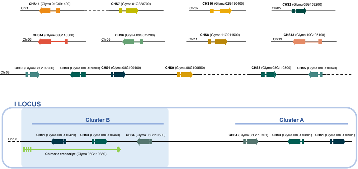
Supplementary Figure 5 | Structure of CHS genes in the Glycine max genome. The structures of all CHS genes are shown with their corresponding locus IDs. The blue box below illustrates the structure of the I locus, including cluster B and A on chromosome 8. The chimeric transcript is present in soybeans with the i^i , i^k , and I alleles, but absent in those with the i allele. Each CHS gene structure is depicted with transcription direction (arrow), exons (thick boxes), and introns (thin boxes). The dotted line represents a condensed depiction of a long genomic distance.
