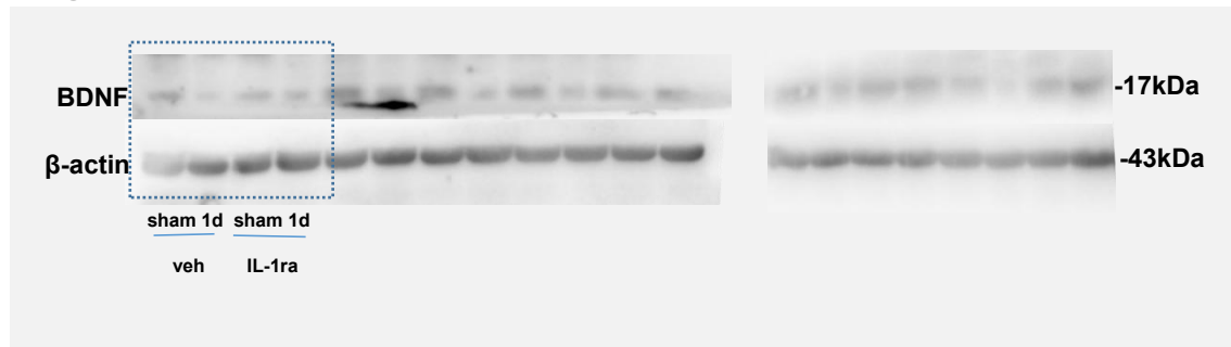
Fig5h BDNF
