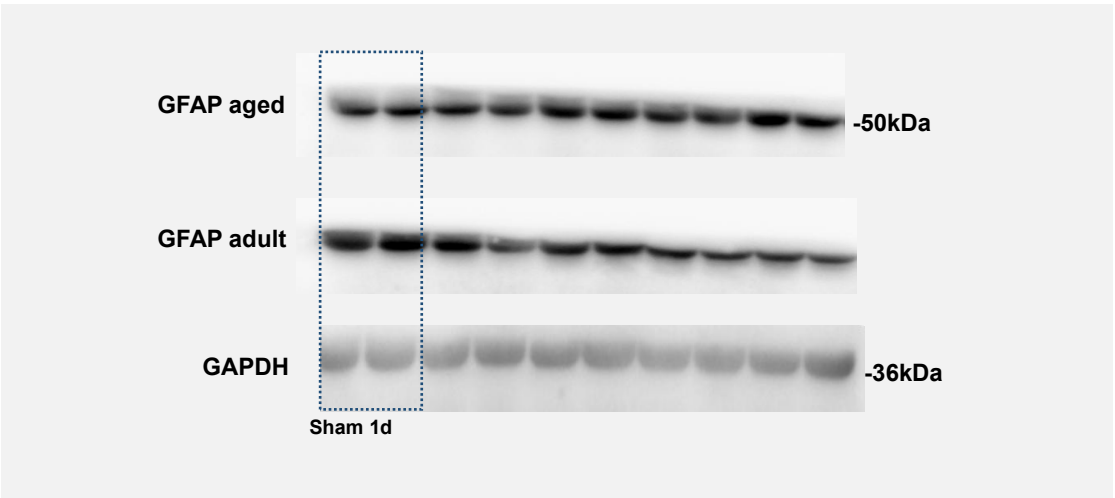
Fig2h GFAP
