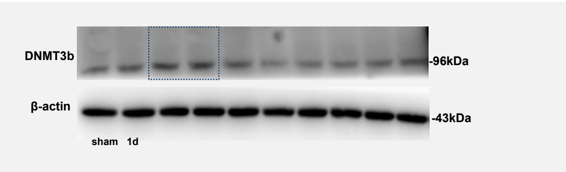
Fig3a DNMT3b
