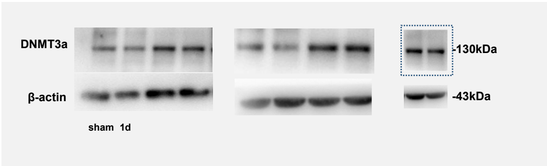
Fig3a DNMT3a
