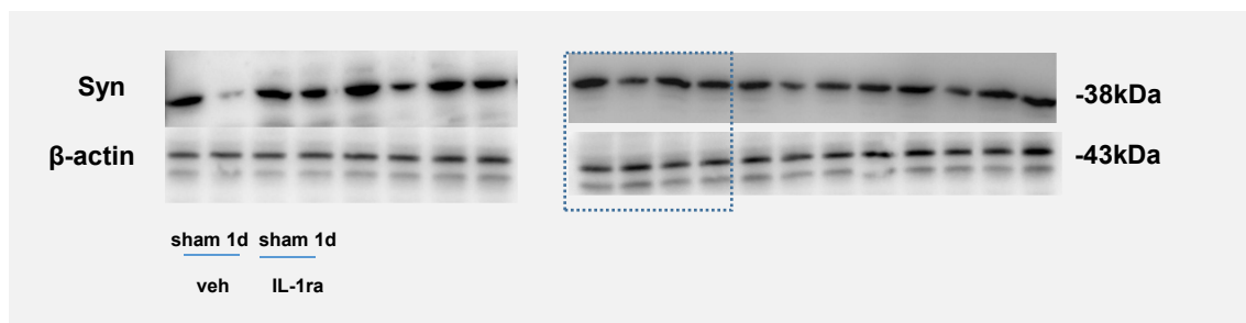
Fig5g Synaptophysin
