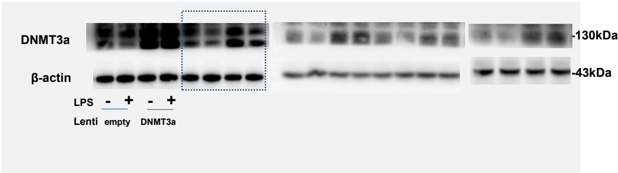
Fig4d DNMT3a
