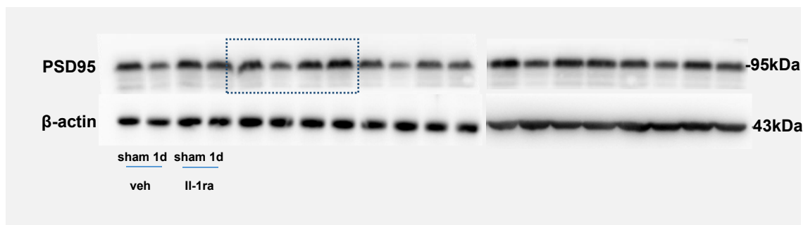
Fig5f PSD95
