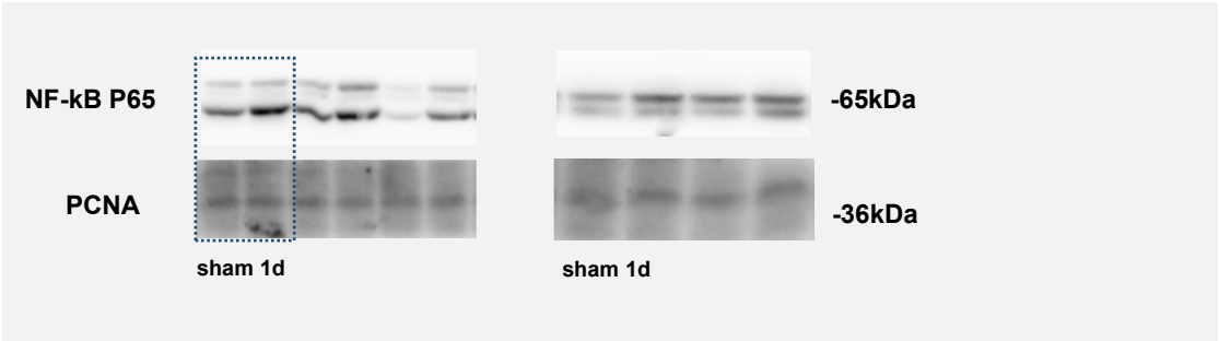
Fig2c NF-kB P65
