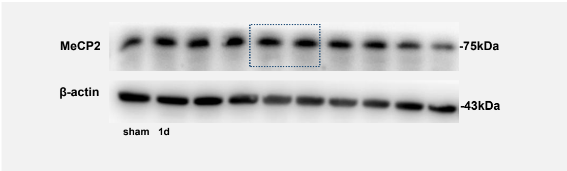
Fig3a MeCP2
