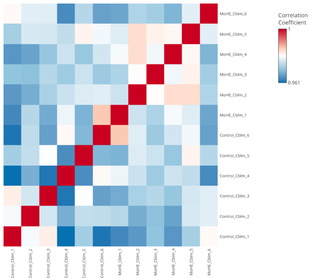
Supplementary Fig. S1 showing the overall correlation heatmap.
